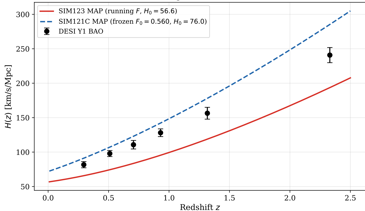
H(z): SIM123 running F vs SIM121C frozen vs DESI
