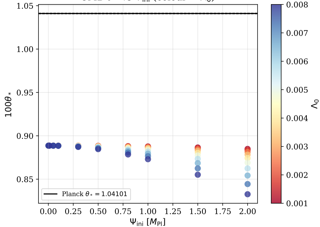
CMB \theta_* vs \Psi_{\text{ini}} (colour = \Lambda_0 )
