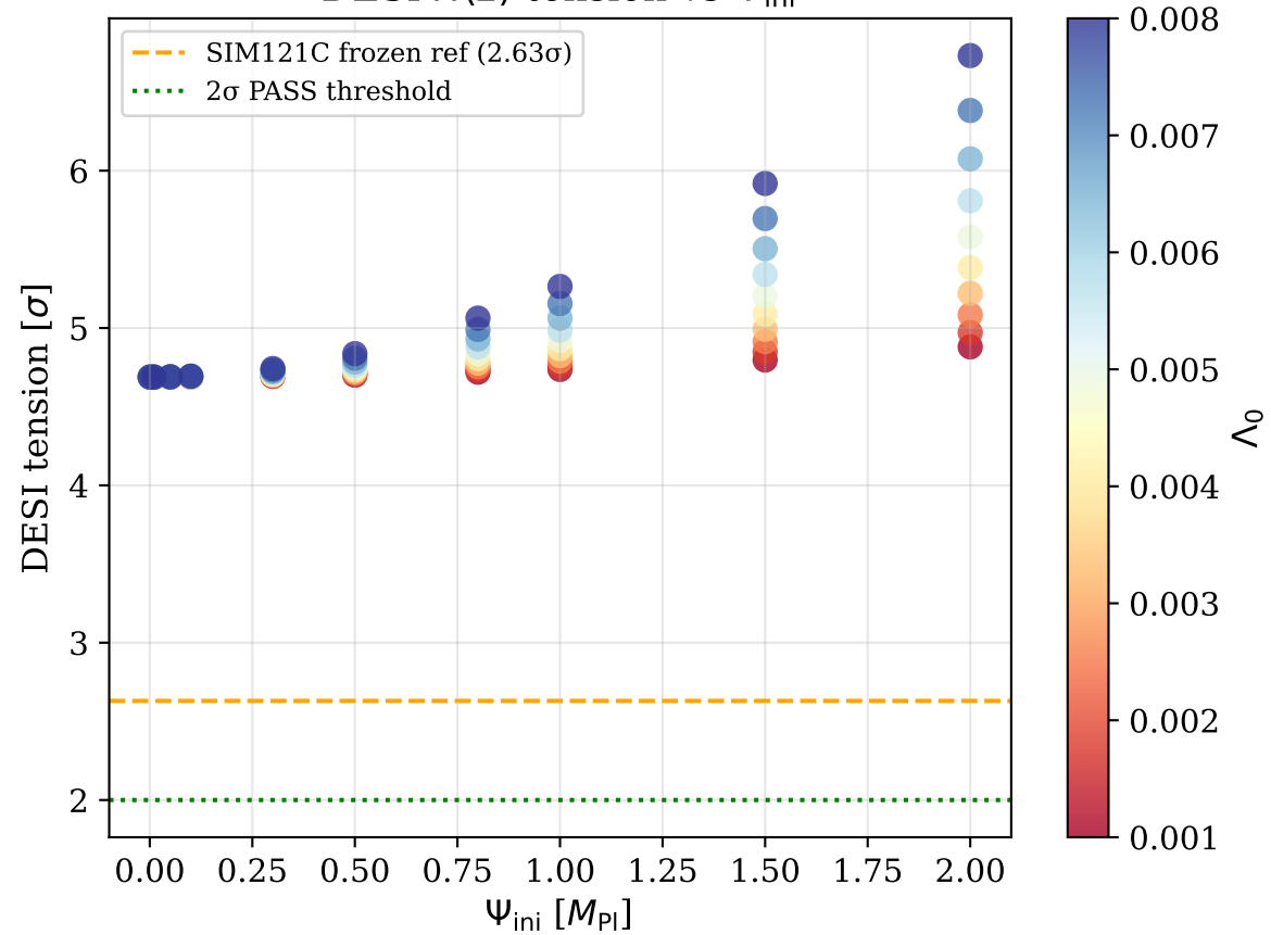
DESI H(z) tension vs \Psi_{\text{ini}}
