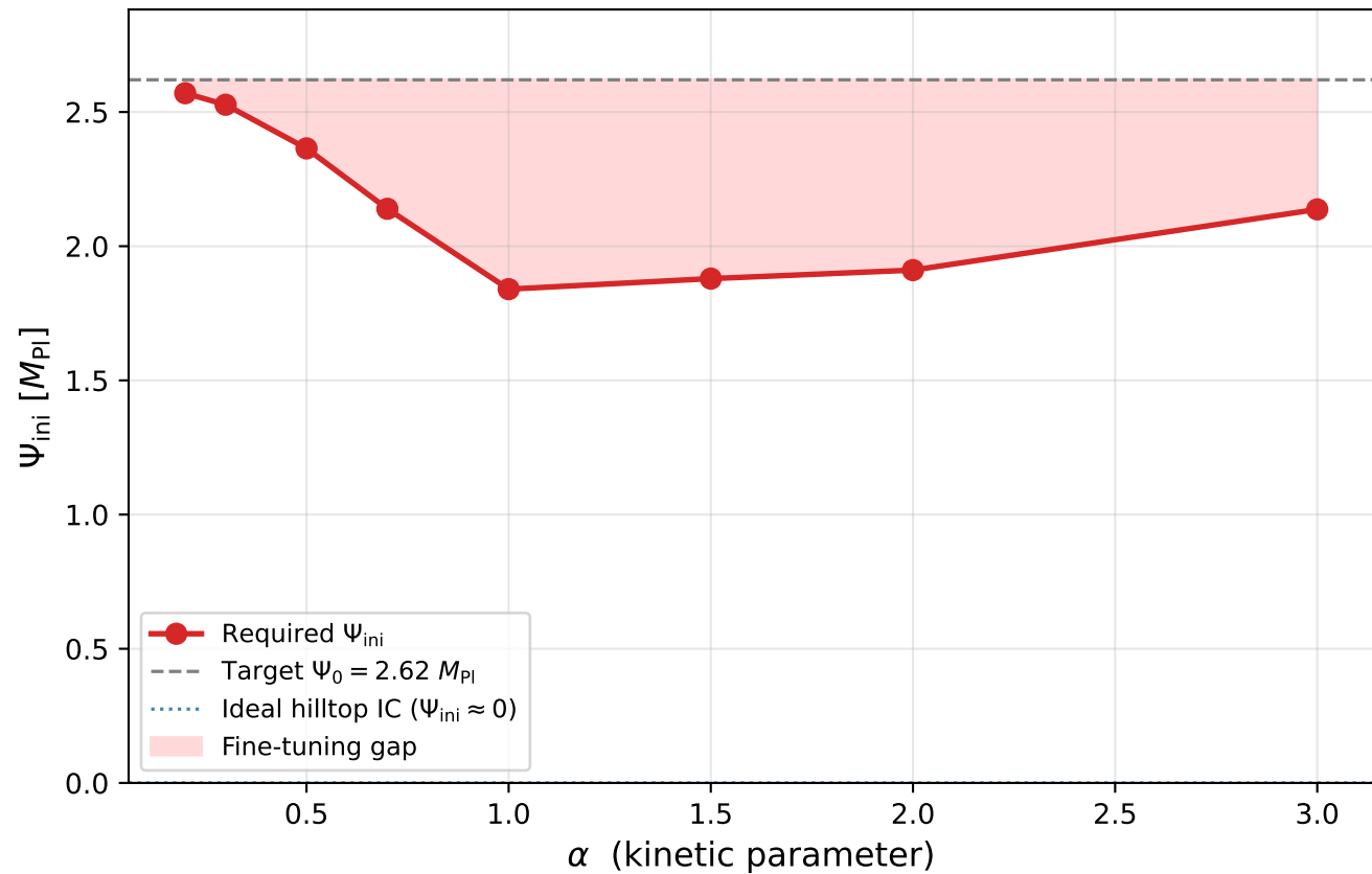
SIM124: Fine-tuning locus — required \Psi_{\text{ini}}(\alpha) to reach \Psi(z=0) = 2.62 M_{\text{Pl}} (true hilltop would give \Psi_{\text{ini}} \approx 0 )
