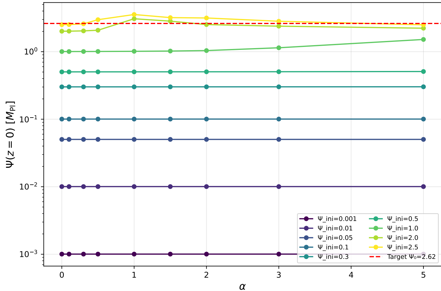
SIM124: Field reached at z=0 vs kinetic parameter \alpha
