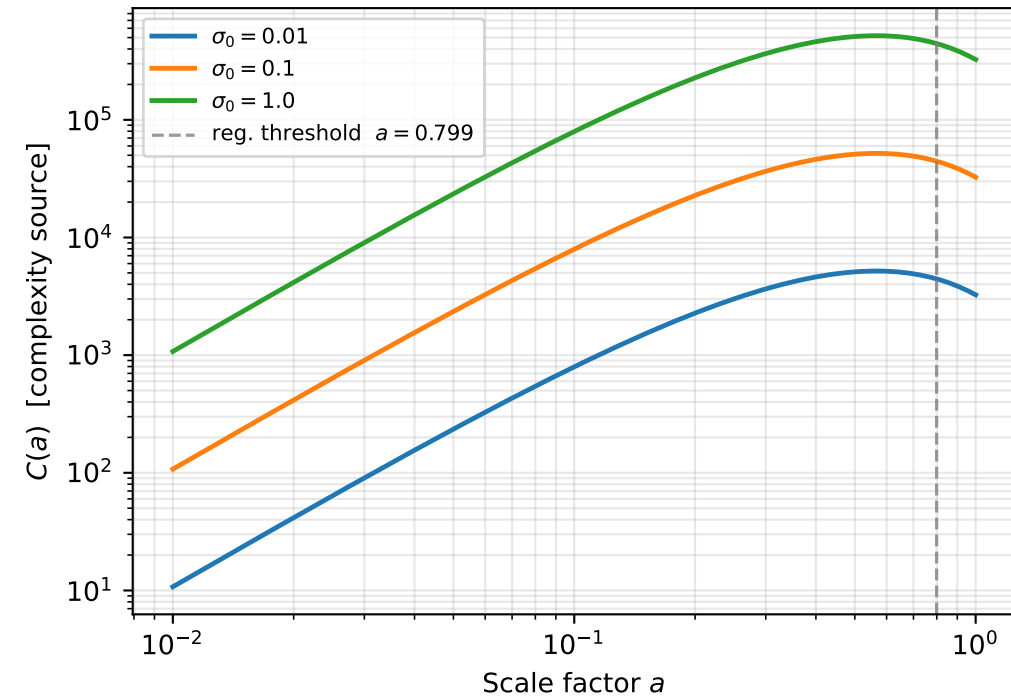
Panel 2 — Complexity Source Term
