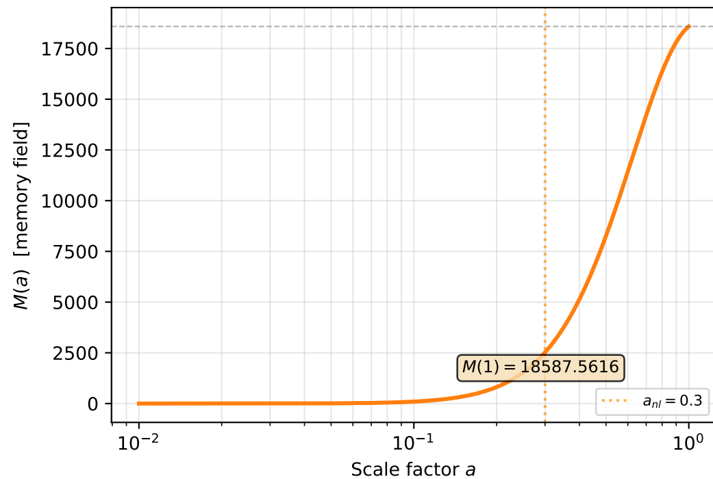
Panel 3 — Memory Field ( \sigma_0 = 0.1 )
