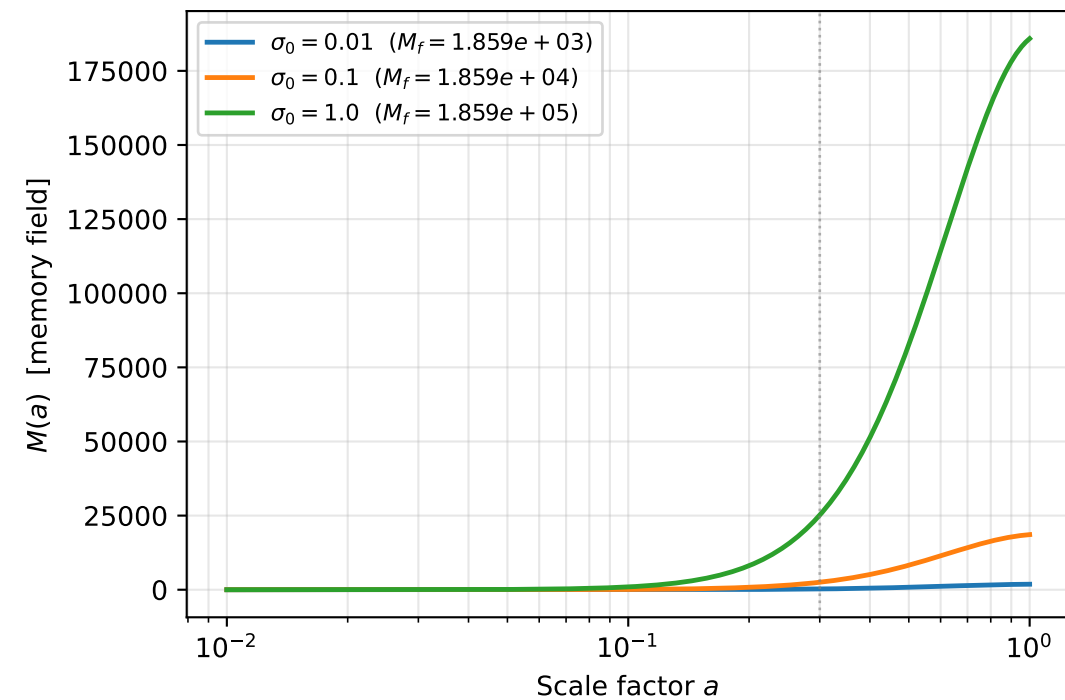
Panel 4 — Memory Field: \sigma_0 Comparison
