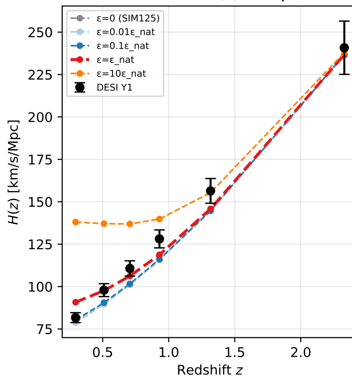
Panel 5 — DESI H(z) Comparison
