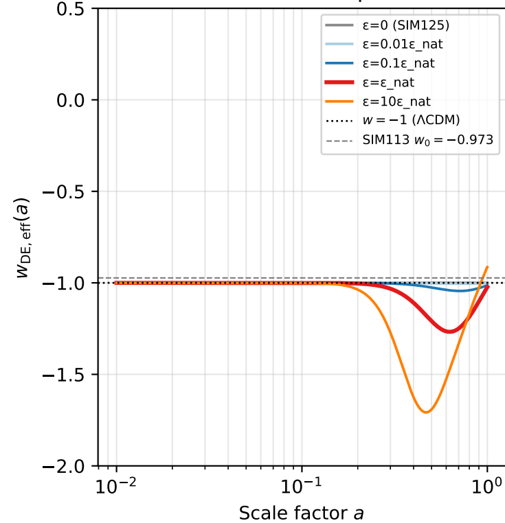
Panel 4 — Effective DE Equation of State
