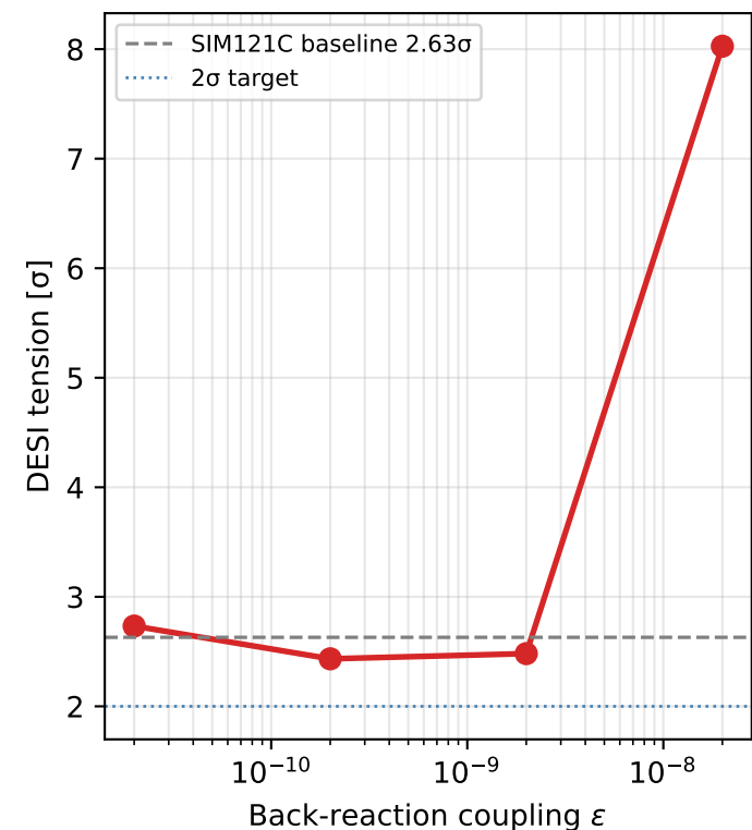
Panel 6 — DESI Tension vs ε
