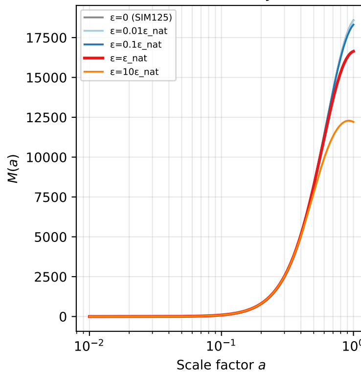
Panel 2 — Memory Field
