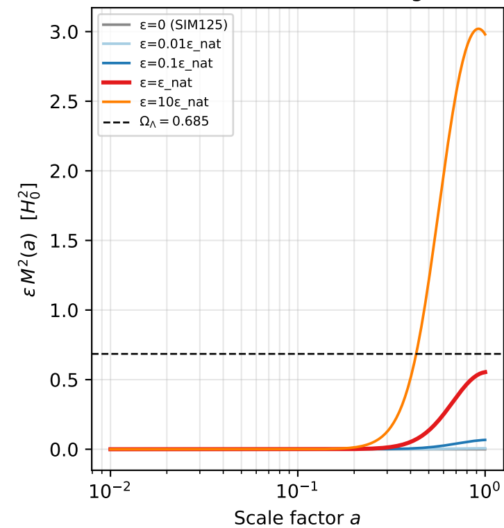
Panel 3 — Back-reaction Magnitude
