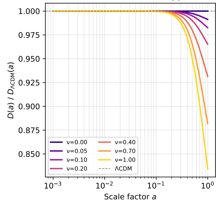
Panel 3 — Growth Factor Suppression
