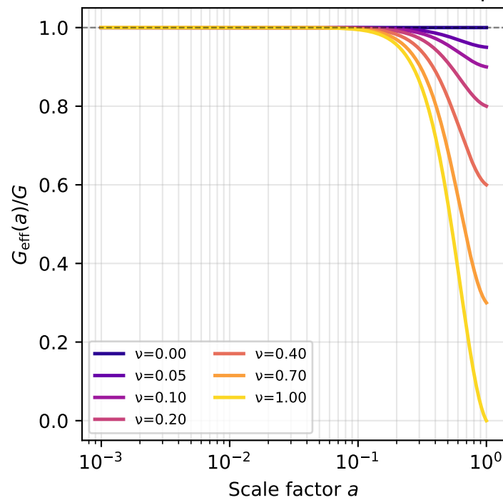
Panel 2 — Effective Gravitational Coupling
