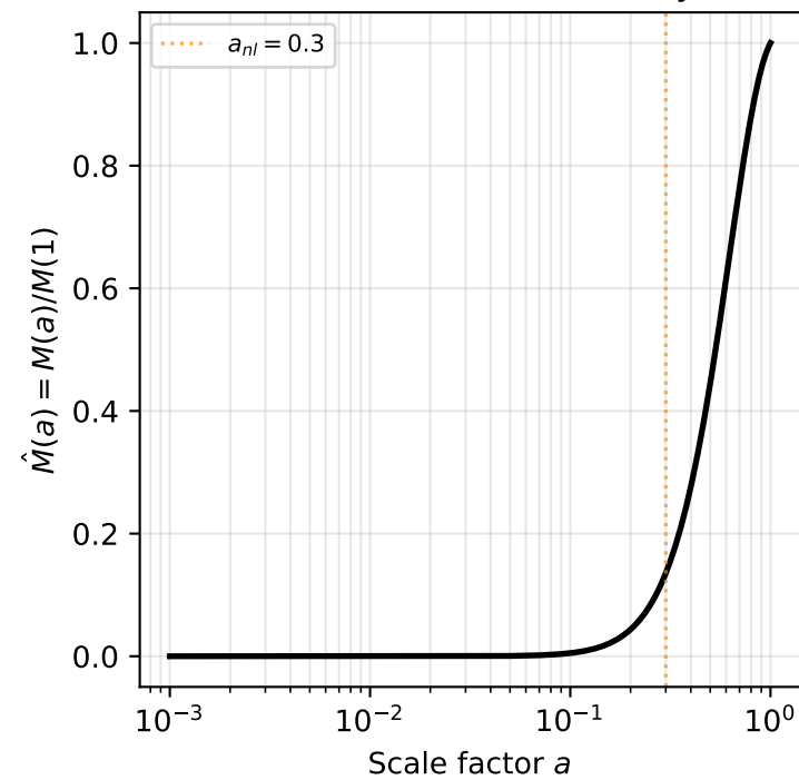
Panel 1 — Normalised Memory Field
