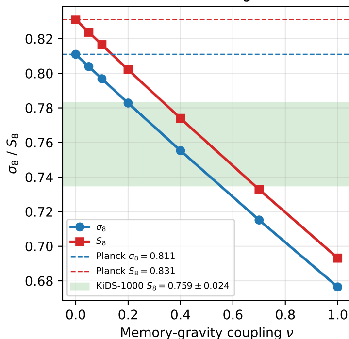
Panel 5 — Tension Diagnostics vs \nu
