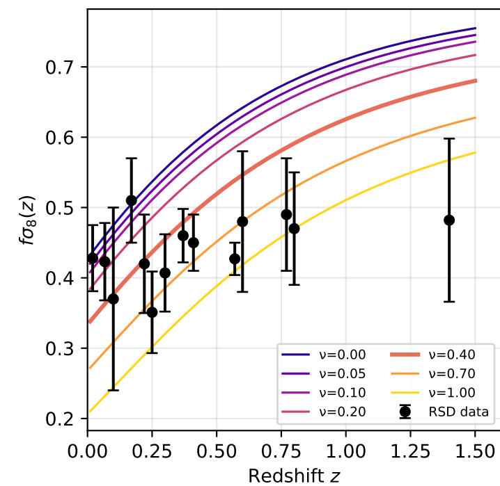
Panel 4 — RSD Growth Rate
