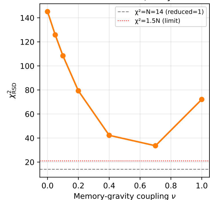
Panel 6 — RSD Fit Quality vs \nu
