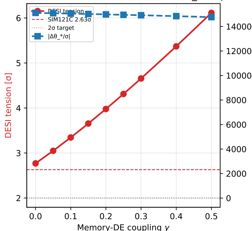
Panel 5 — DESI Tension and CMB \theta_* vs \gamma
