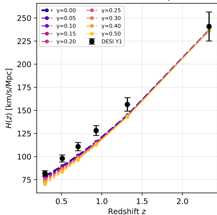
Panel 4 — DESI H(z) Comparison
