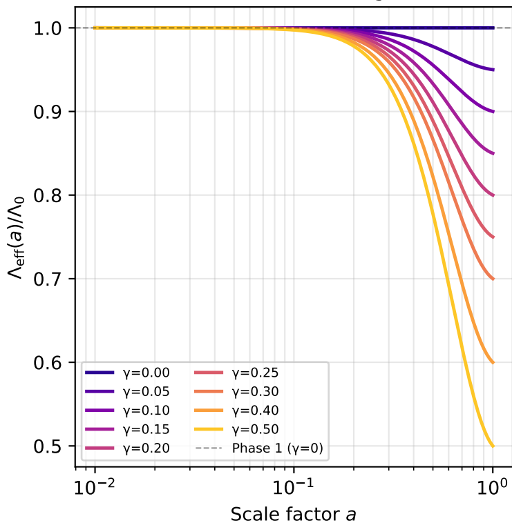
Panel 1 — Effective Cosmological Constant
