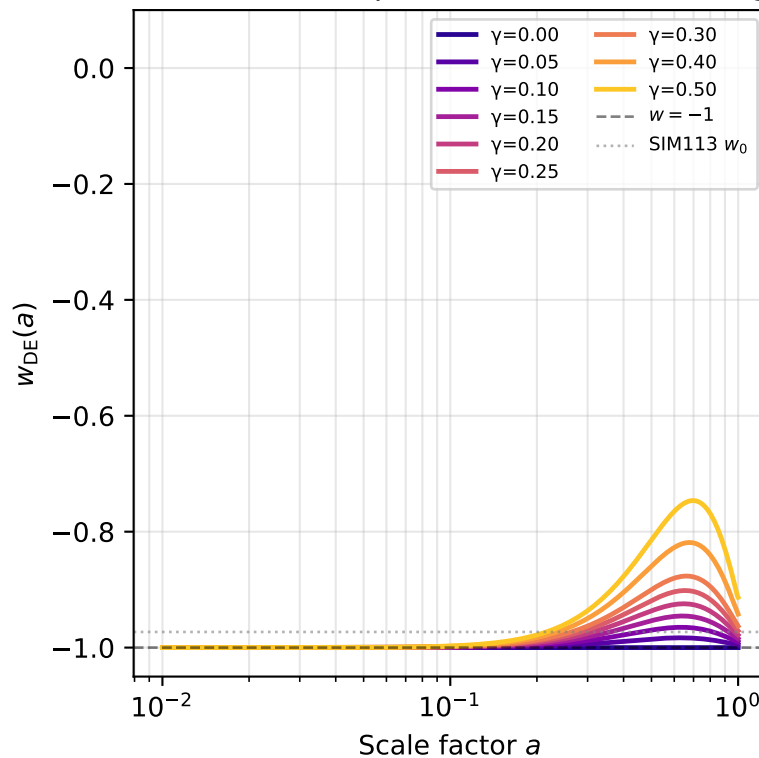
Panel 2 — DE Equation of State (thawing)
