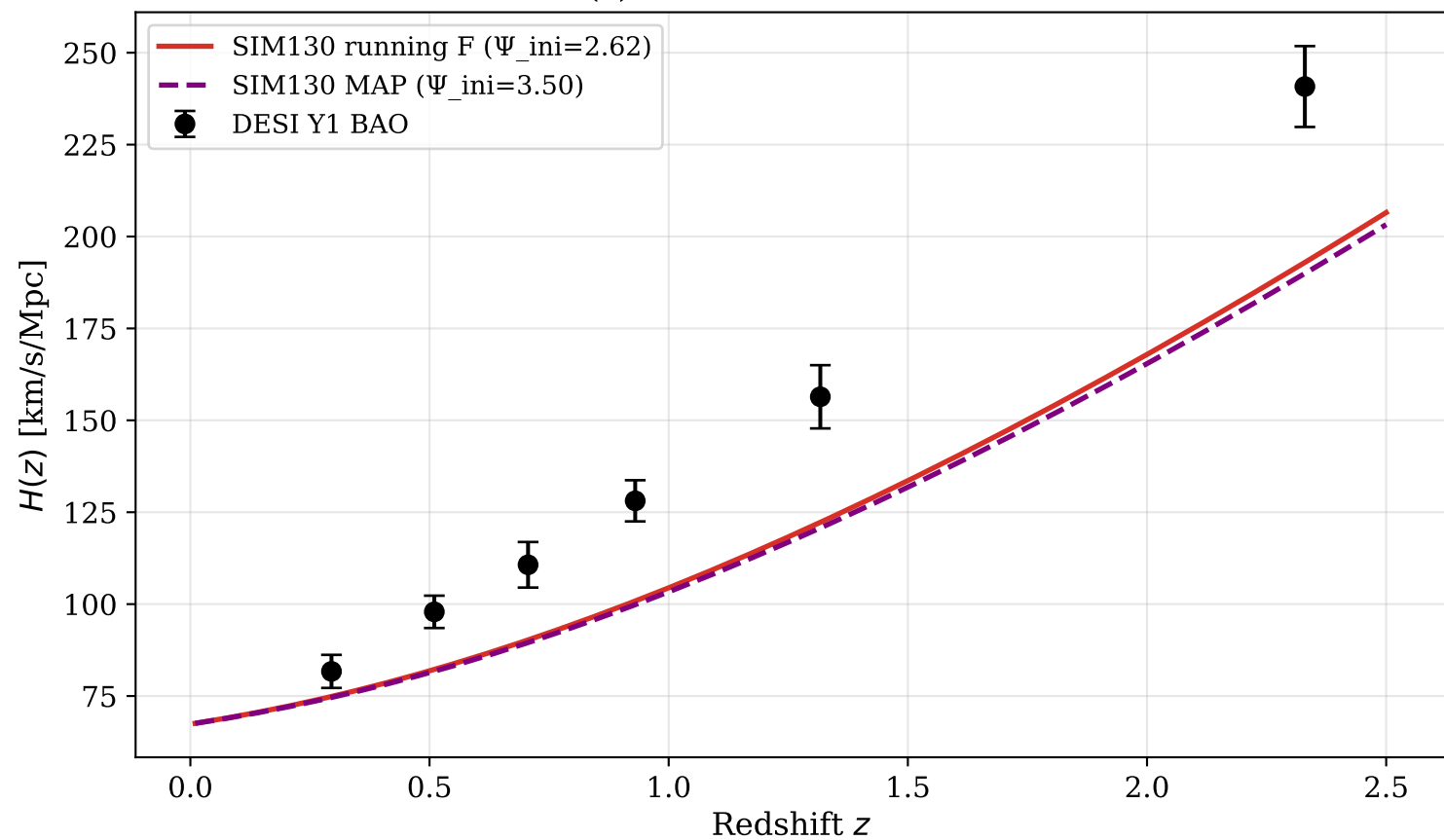
SIM130: H(z) — unlocked Phase 1 \Psi vs DESI
