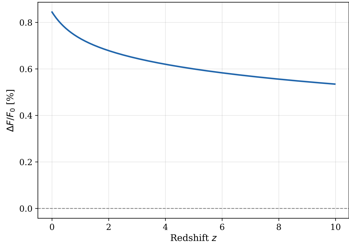
Fractional F(z) change (drives \Delta H/H )
