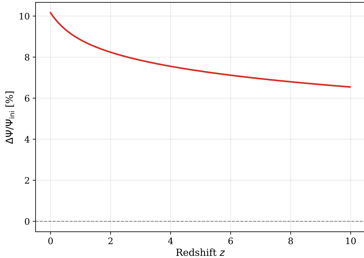
Fractional \Psi change from curvature sourcing
