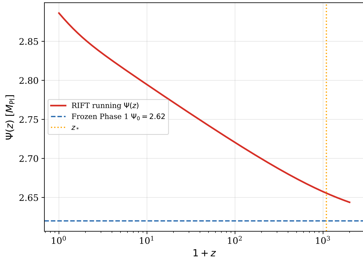
\Psi(z) — curvature-sourced evolution (Phase 1)
