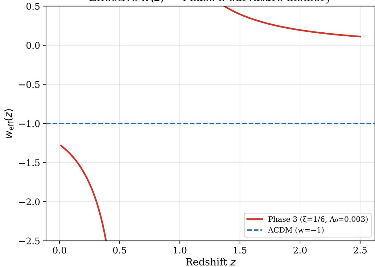
Effective w(z) — Phase 3 curvature memory
