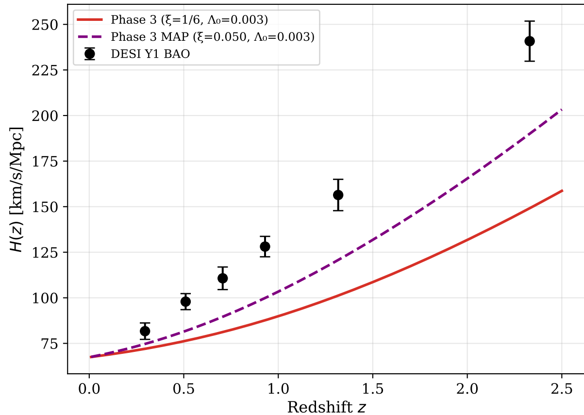
Phase 3 H(z) vs DESI
