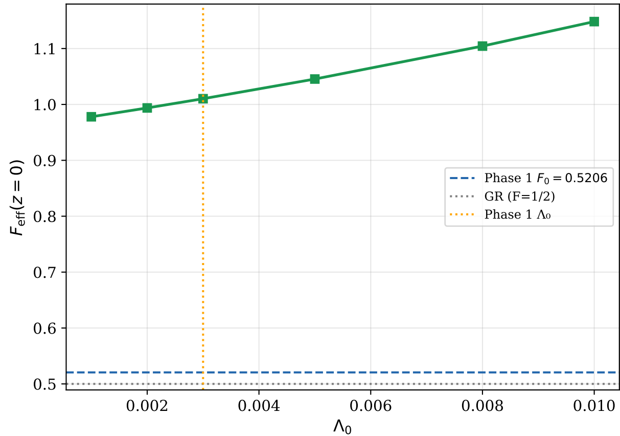
F_{\text{eff},0} vs \Lambda_0
