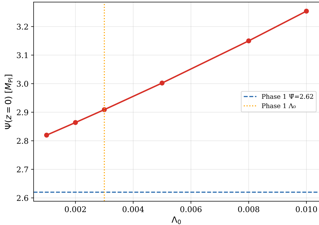
Today's \Psi_0 vs \Lambda_0 ( \xi=1/6 , \Psi_{\text{ini}}=0 )
