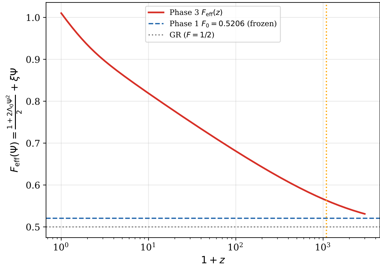
Running F_{\text{eff}}(z) — Phase 3 vs Phase 1
