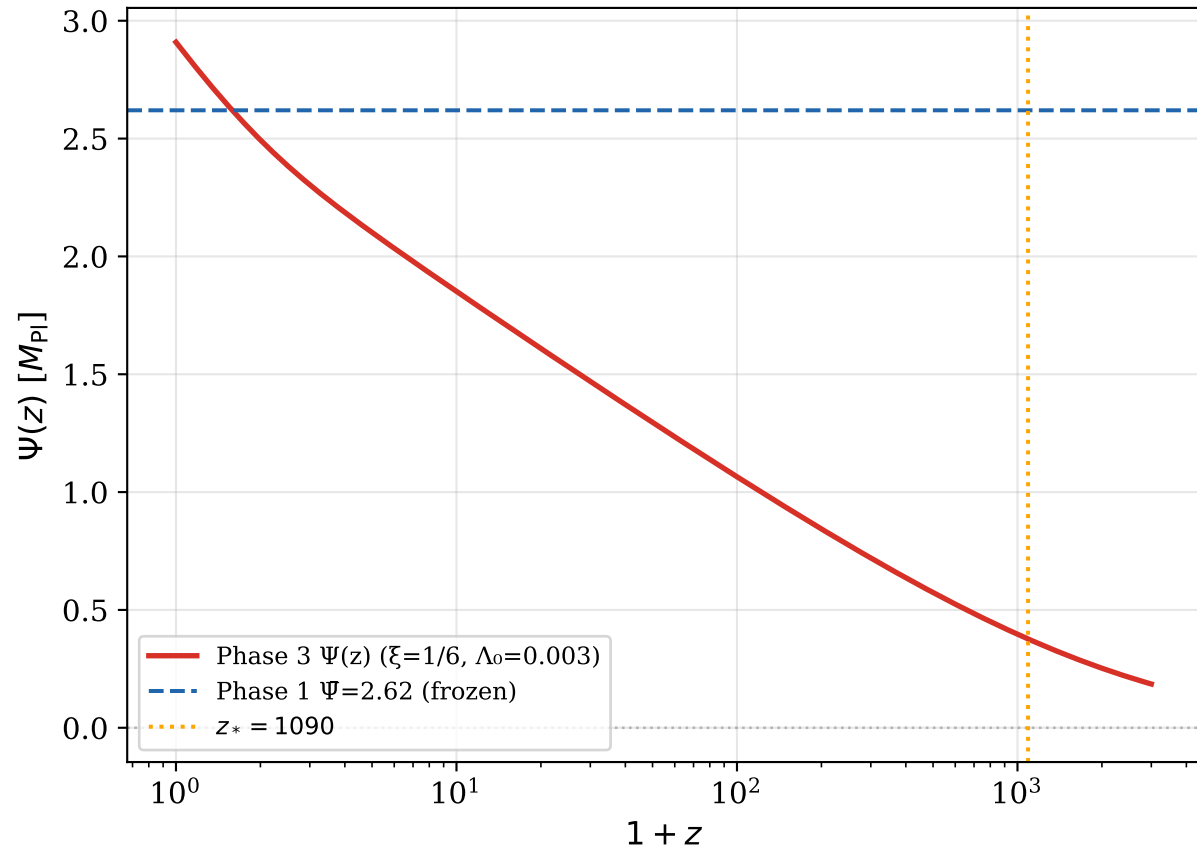
Phase 3: Curvature-memory \Psi(z) from \Psi_{\text{ini}} = 0
