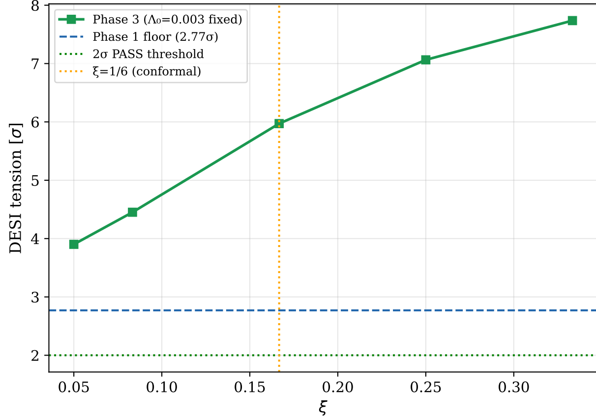
DESI tension vs \xi ( \Lambda_0 = 0.003 )
