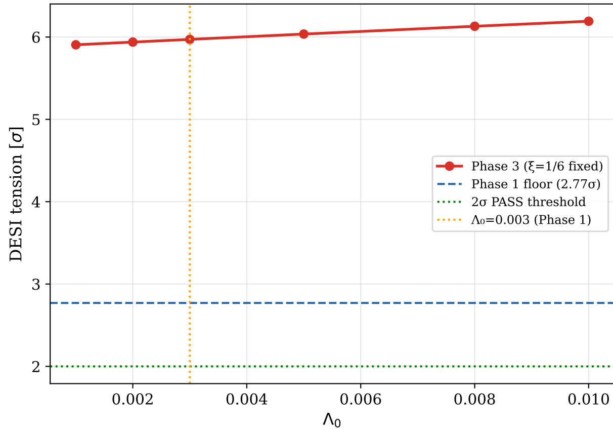
DESI tension vs \Lambda_0 ( \xi=1/6 )
