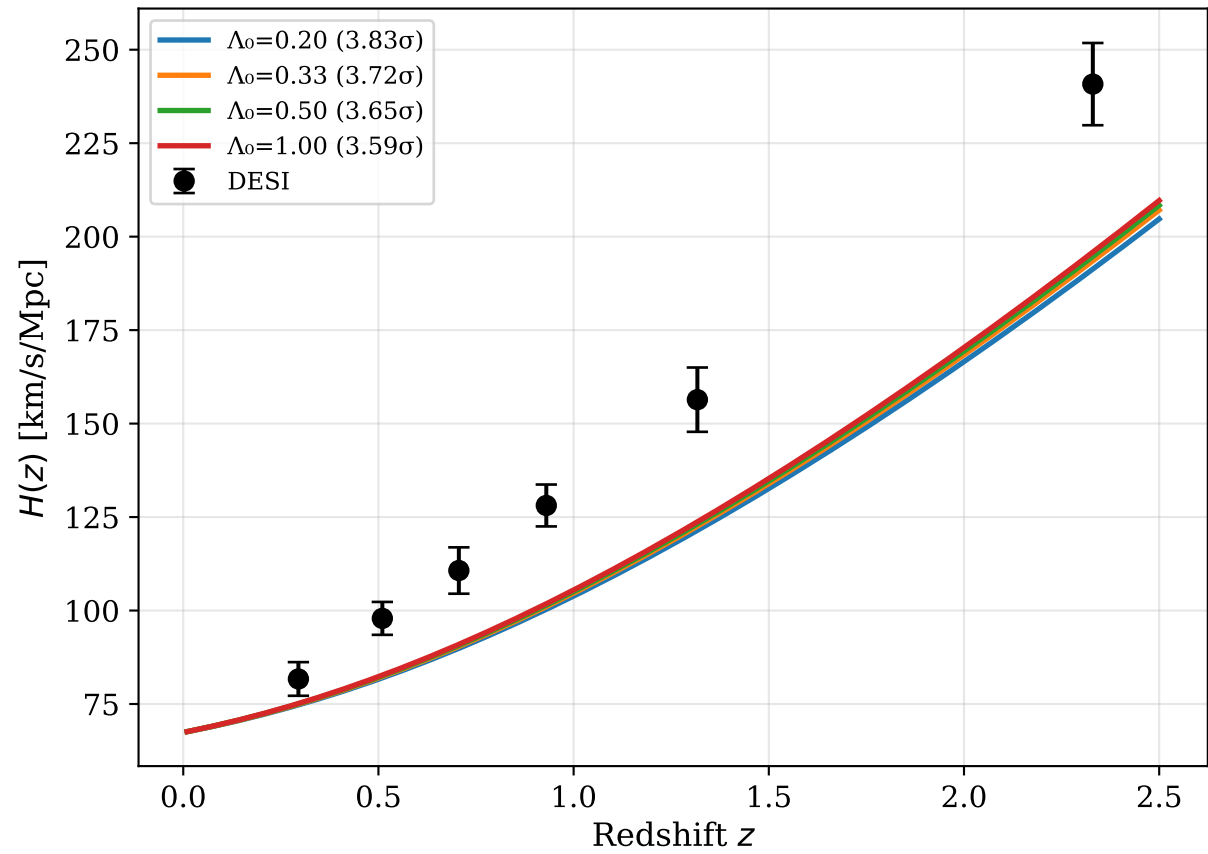
SIM132: H(z) vs DESI
