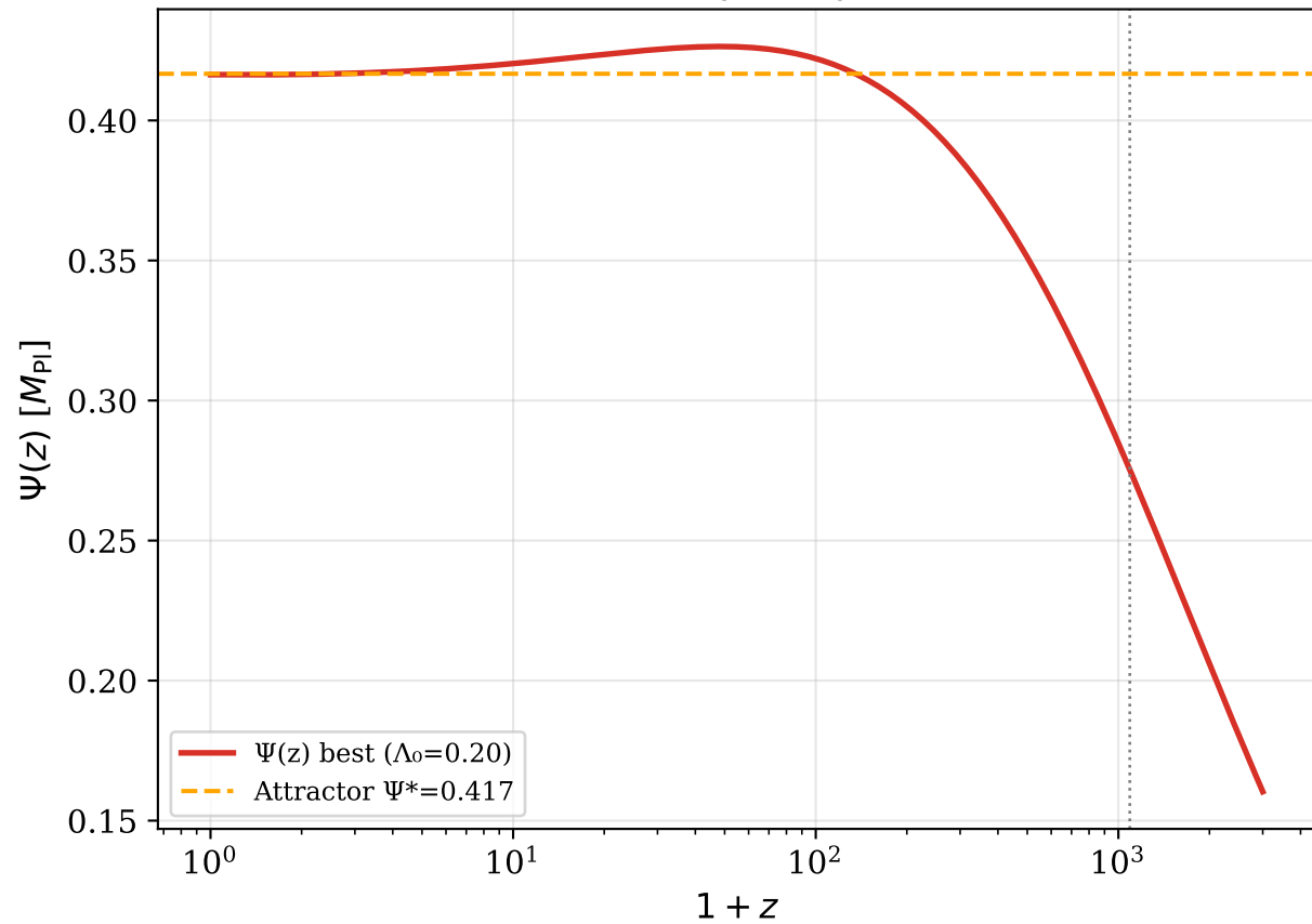
SIM132: Field trajectory to attractor
