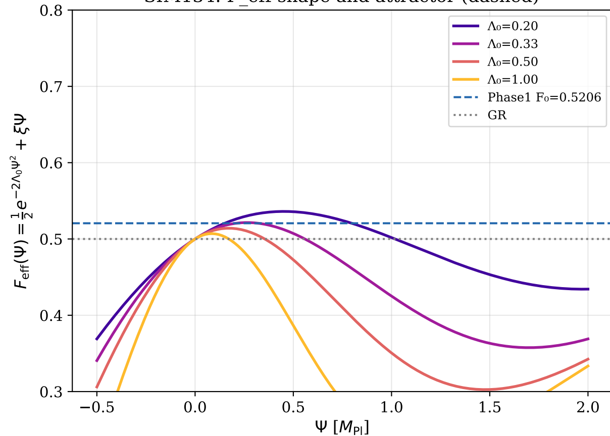
SIM134: F_eff shape and attractor (dashed)
