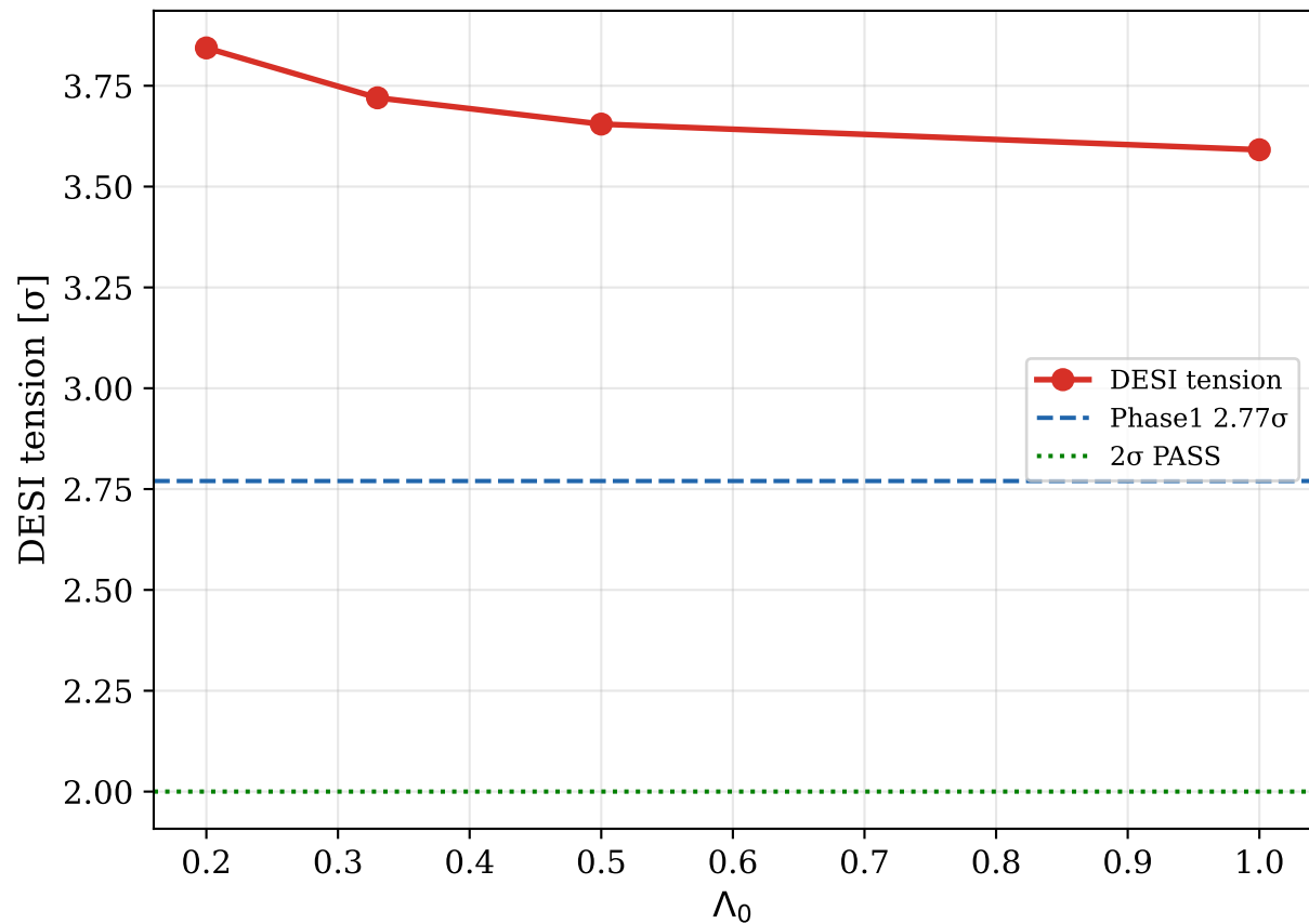
SIM134: DESI tension vs \Lambda_0
