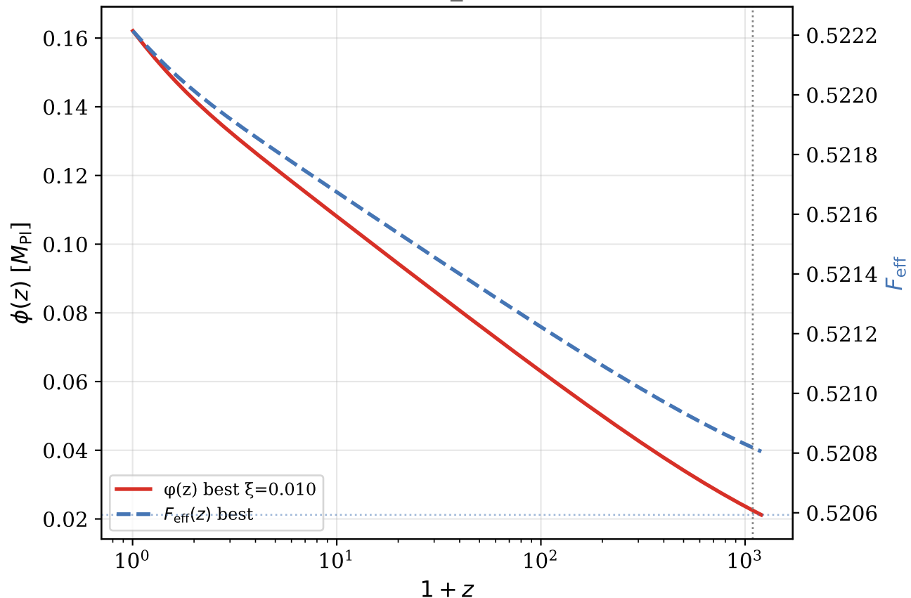
SIM135: Field and F_{\text{eff}} evolution (best)
