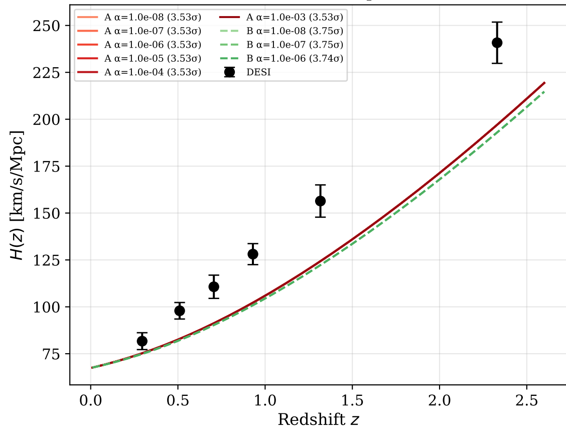
SIM136: H(z) comparison
