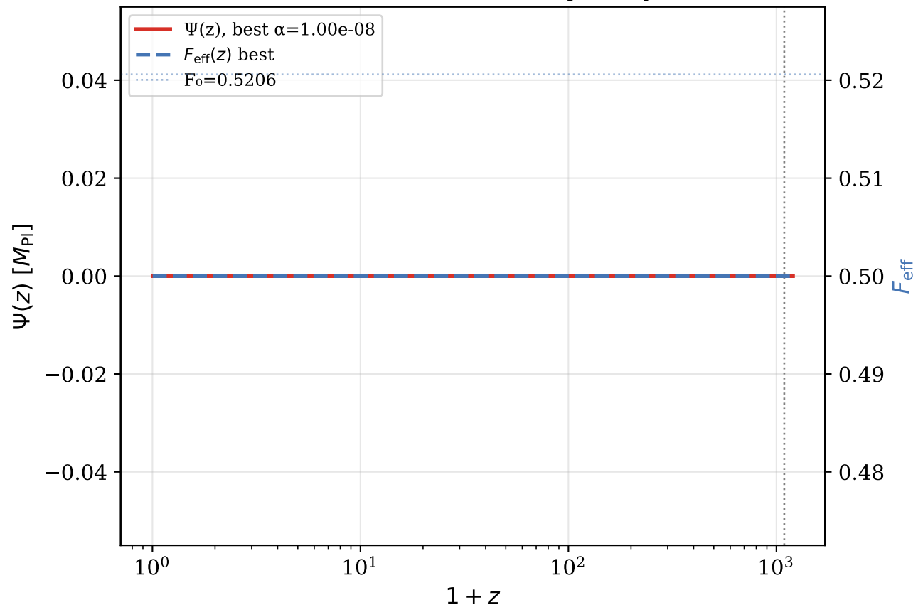
SIM136: Best field trajectory
