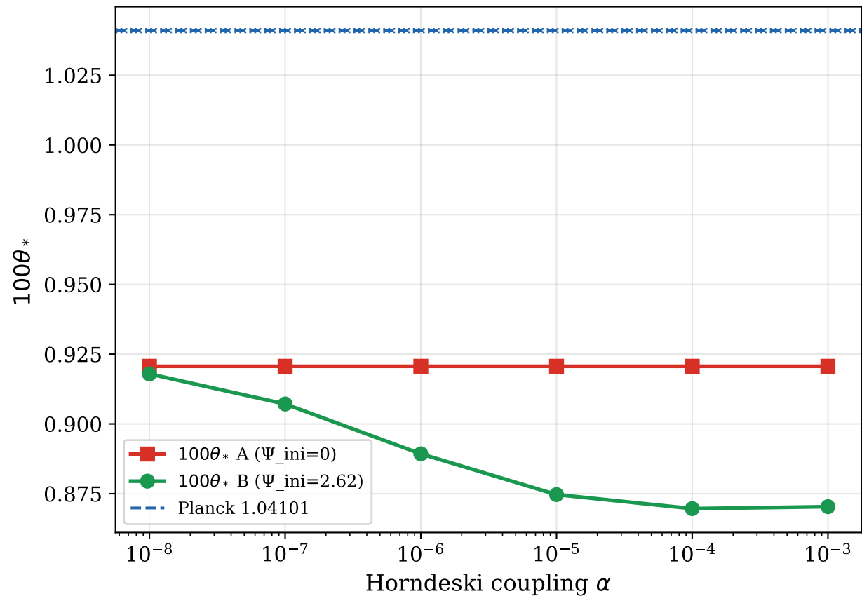
SIM136: CMB acoustic scale vs Horndeski \alpha
