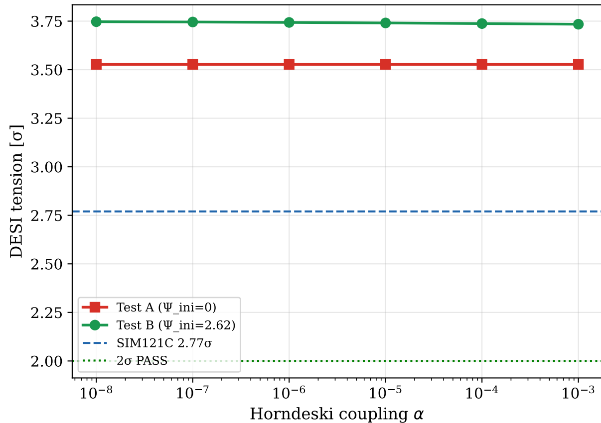
SIM136: DESI tension vs Horndeski \alpha
