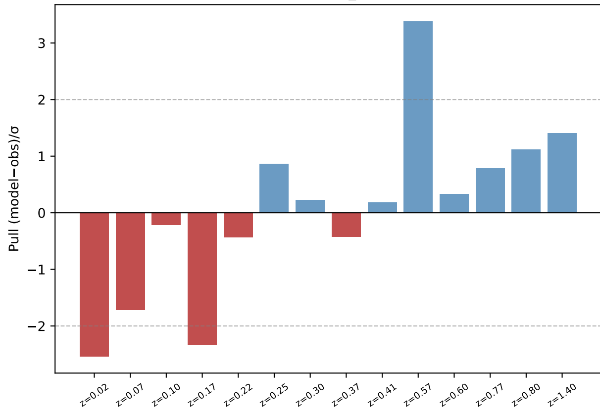
SIM139: Per- z pulls Verdict: SHAPE_FIXABLE
