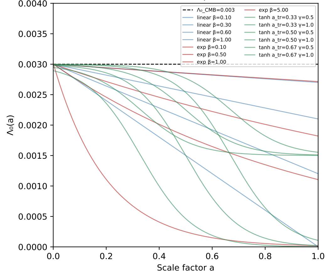
SIM141: \Lambda_0(a) profiles
