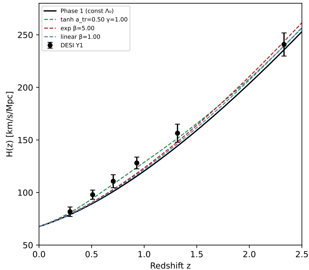
SIM141: H(z) best cases
