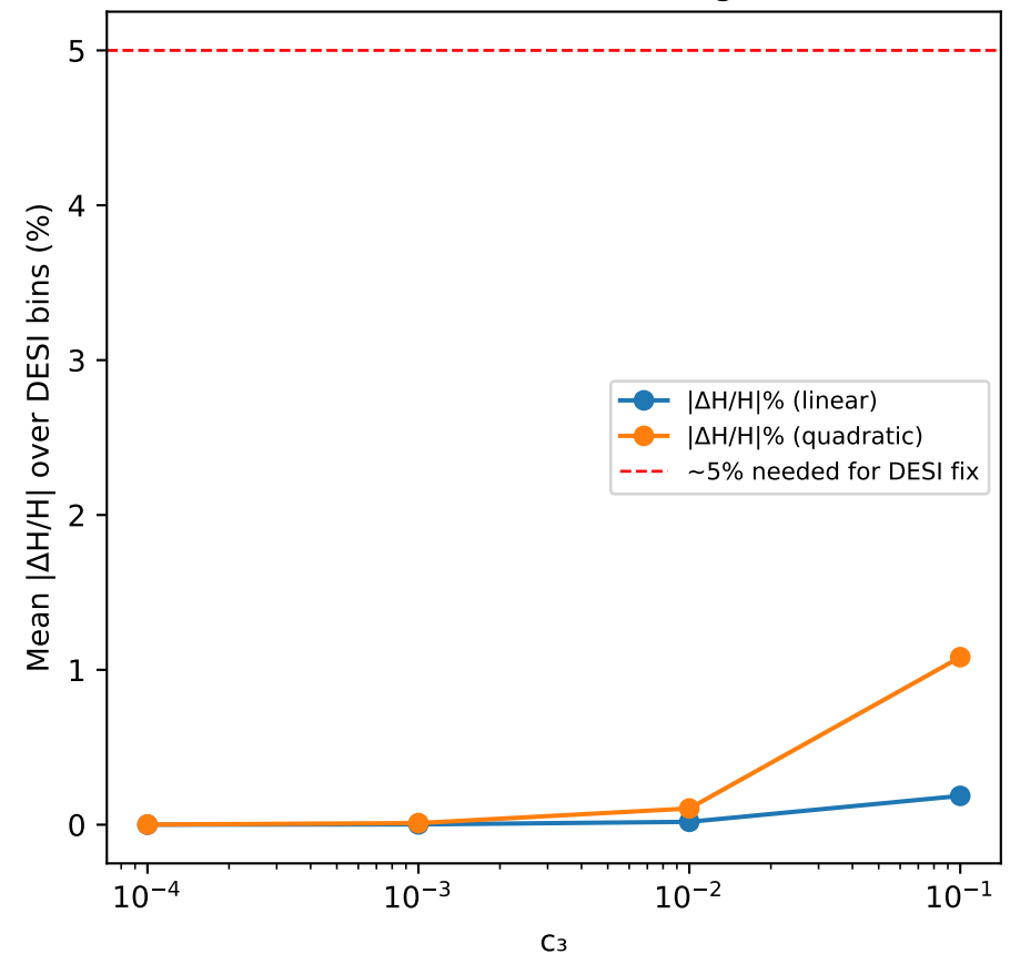
SIM142: G_3 correction magnitude
