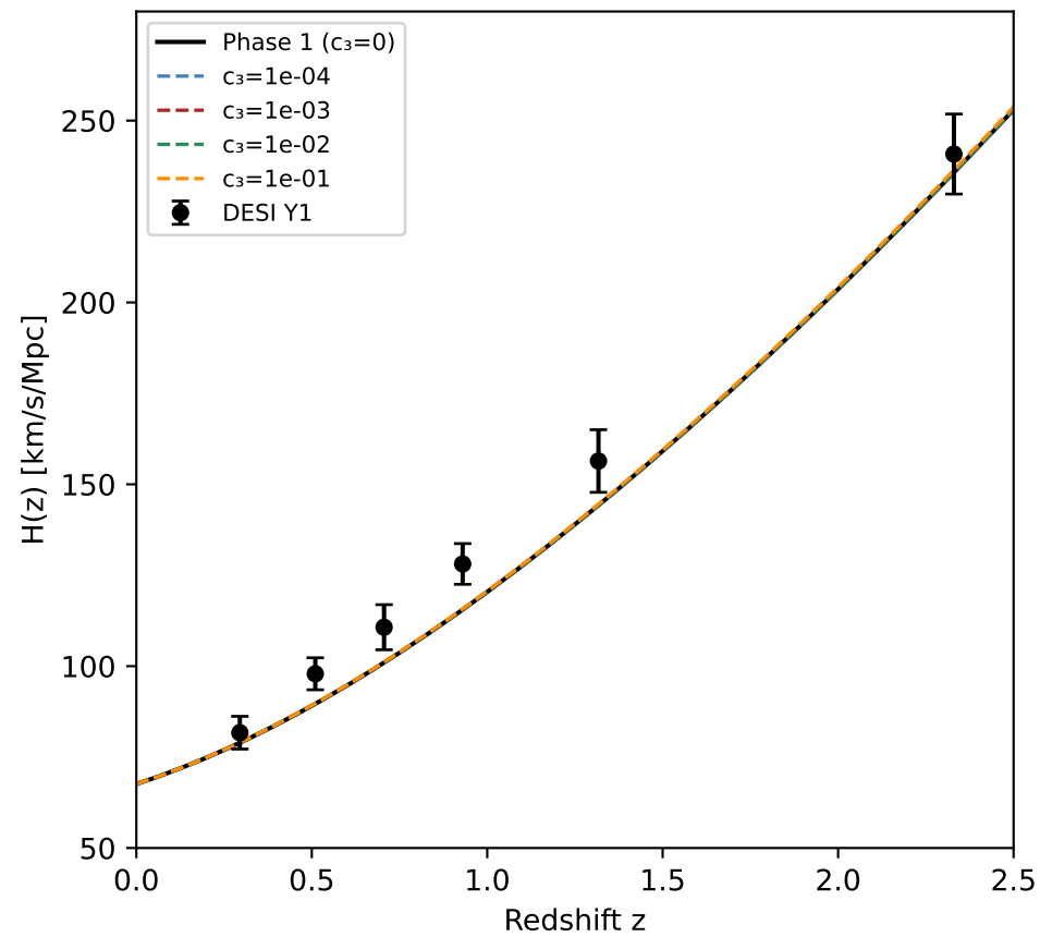
SIM142: H(z) — linear G_3
