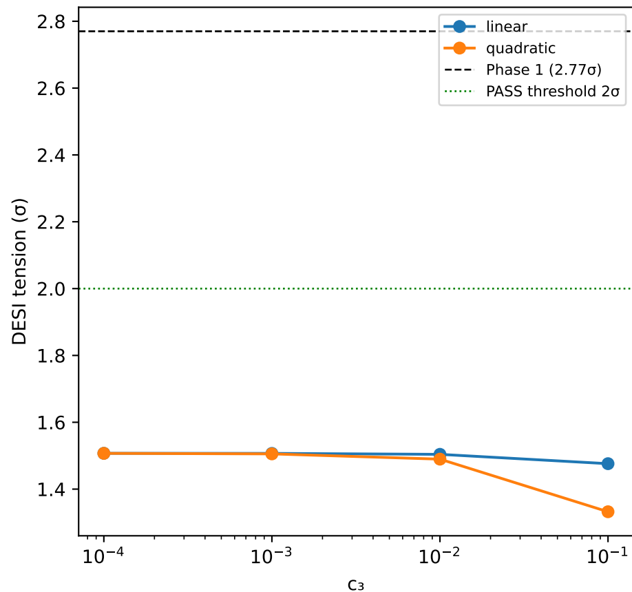
SIM142: DESI tension vs c_3
