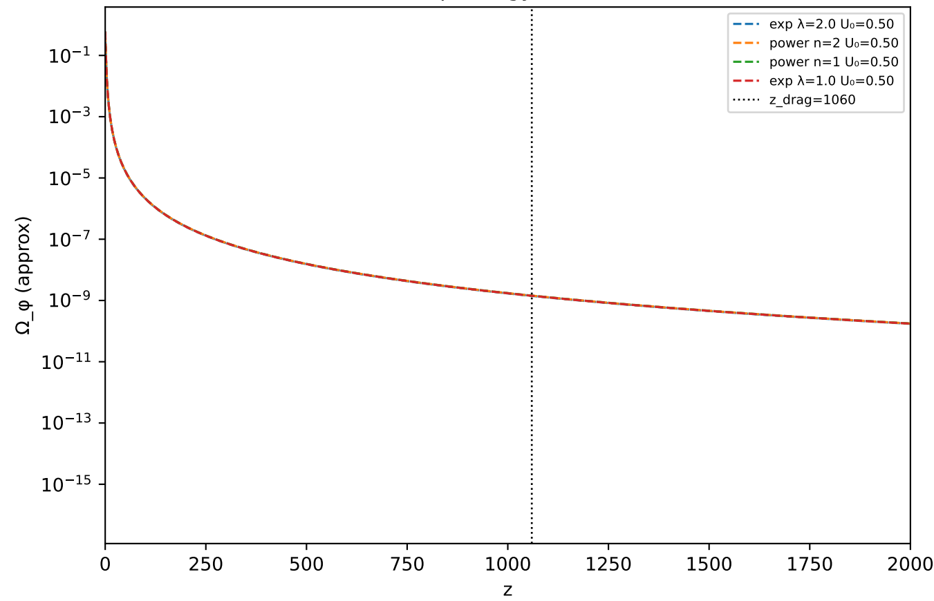
SIM143: \phi energy fraction vs z
