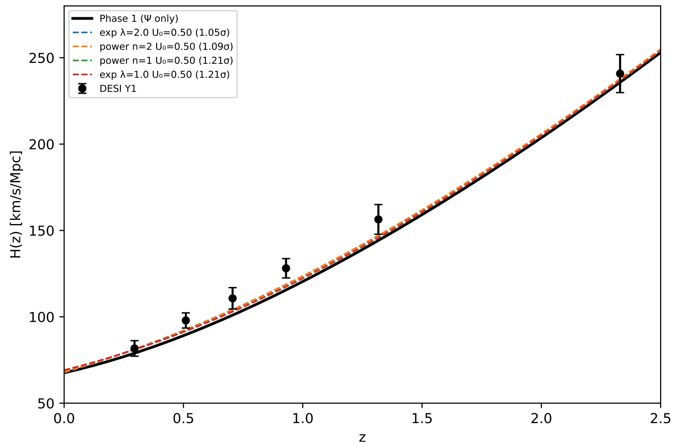
SIM143: H(z) — best DESI cases
