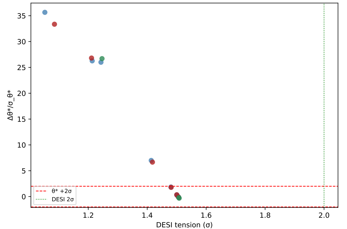
SIM143: DESI vs CMB (anti-correlation?)
