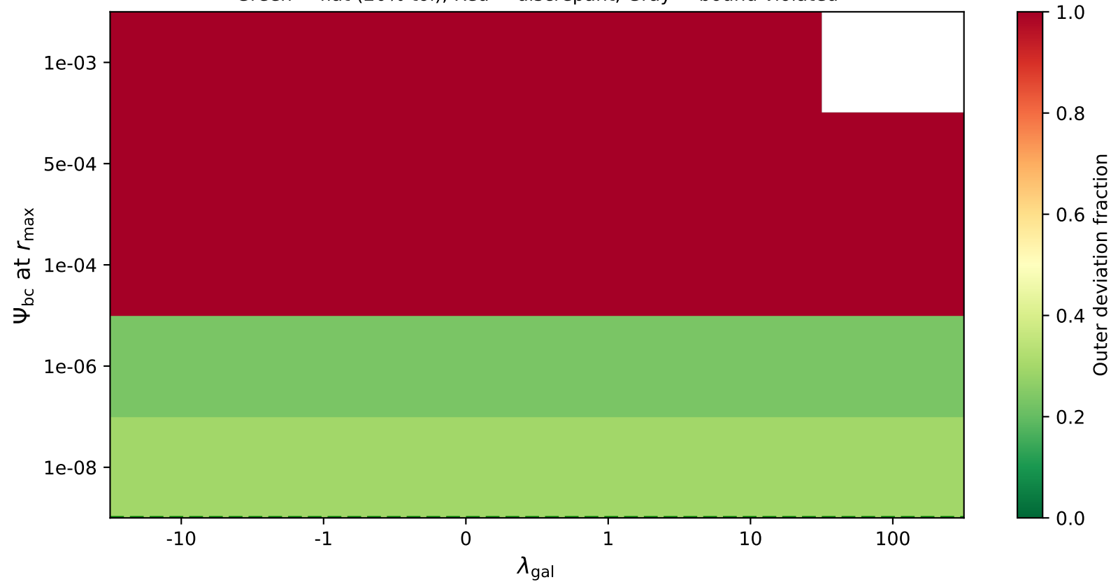
NGC6503 — Outer |v_c - v_{flat}|/v_{flat} (within cosmo+energy bounds) Green = flat (20% tol), Red = discrepant, Gray = bound violated
