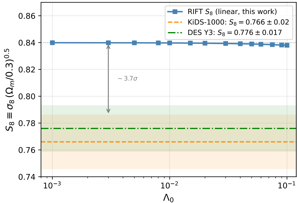
S_8 Tension: RIFT vs Observations (linear \sigma_8 )
