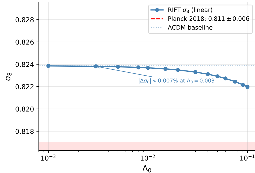
\sigma_8 vs Coupling Strength
