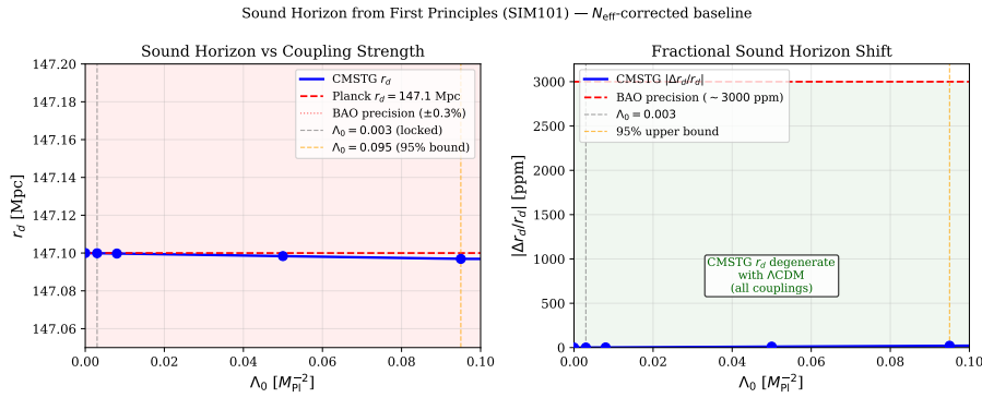
Figure 9: Sound horizon r_d as a function of \Lambda_0 (SIM101), with the N_{\text{eff}} -corrected LCDM baseline anchored at r_d^{\text{Planck}} = 147.1 Mpc. Across the entire allowed range \Lambda_0 \in [0, 0.095] , the maximum fractional shift is |\Delta r_d/r_d| = 21 ppm, compared to current BAO measurement precision of \sim 0.3\% (3000 ppm). CMSTG and \Lambda CDM are degenerate in r_d at all observationally allowed couplings.
