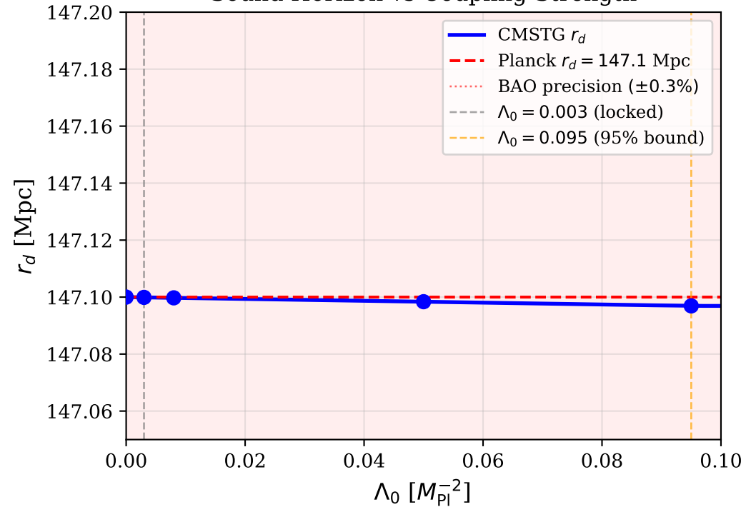
Sound Horizon vs Coupling Strength
