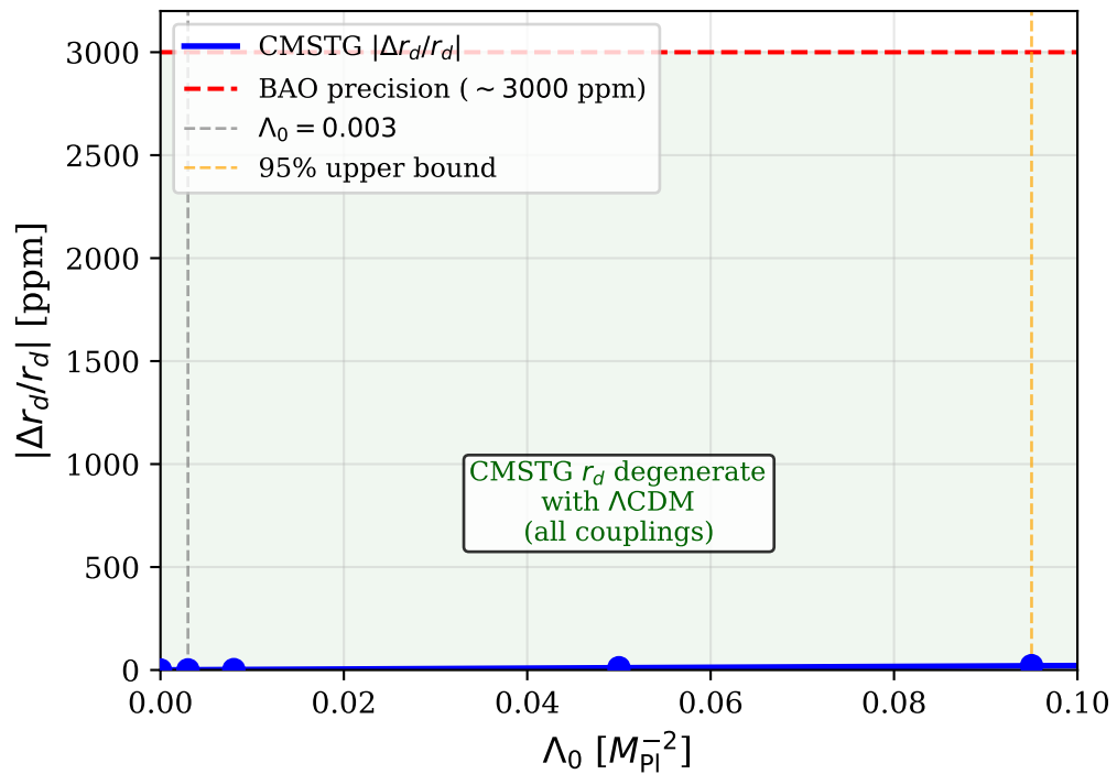
Fractional Sound Horizon Shift
