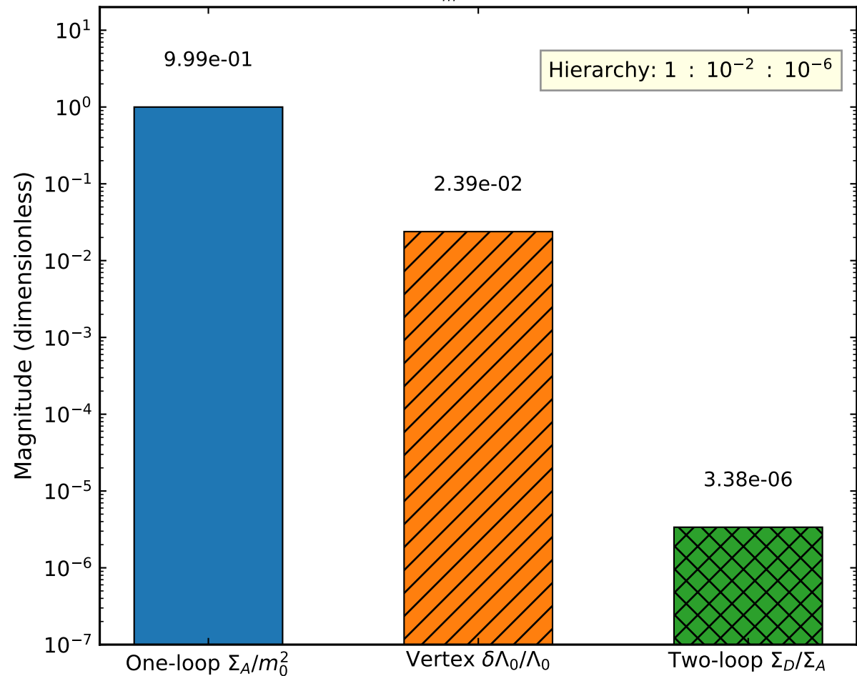
Perturbative hierarchy at k_m^{\text{nat}} = 9.15 \text{ Mpc}^{-1} (SIM104/SIM106)
