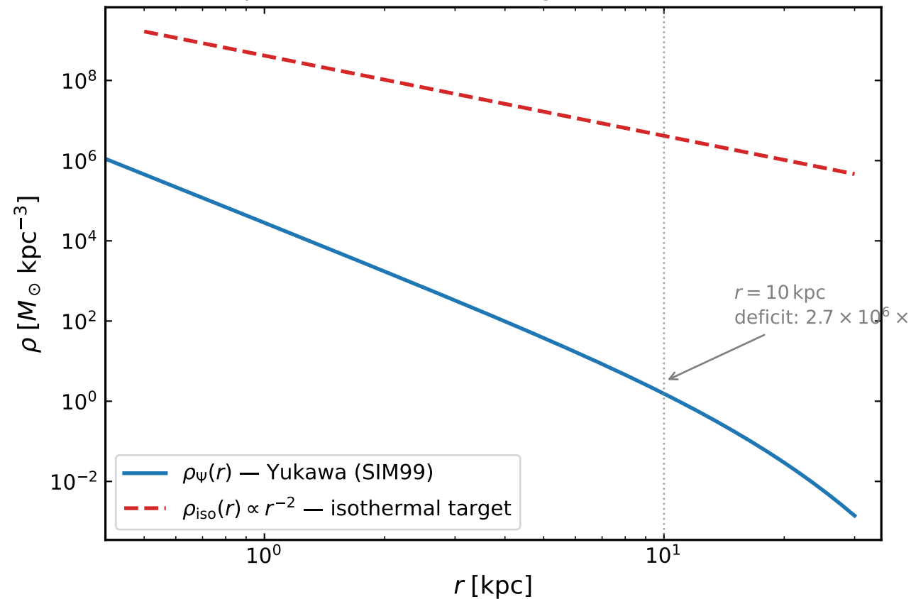
SIM99 — Yukawa profile vs isothermal target (NGC\,3198, v_{\text{flat}} = 150 \text{ km s}^{-1} )
