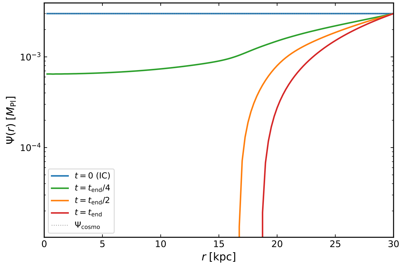
SIM100 — Time-domain \Psi(r, t) evolution
