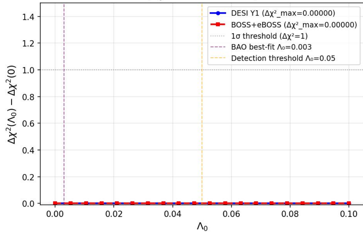
\Lambda_0 Sensitivity: DESI Y1 vs BOSS+eBOSS (at joint CMB+BAO best-fit)
