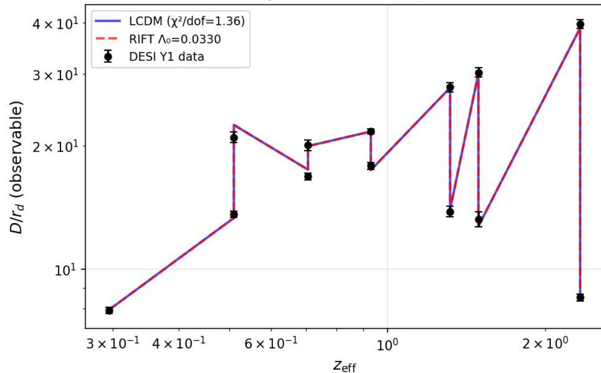
DESI Y1 BAO: LCDM vs RIFT predictions (joint CMB+BAO best-fit)
