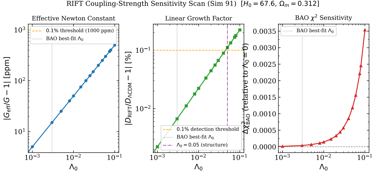
Figure 7: RIFT coupling-strength sensitivity scan (Sim 91) at the joint CMB+BAO best-fit cosmology ( H_0 = 67.6 , \Omega_m = 0.312 ). Left : |G_{\text{eff}}/G - 1| in ppm; the dashed orange line marks the 0.1% ( 10^3 ppm) strong-lensing detection threshold. Centre : linear growth factor deviation |D_{\text{RIFT}}/D_{\Lambda\text{CDM}} - 1| ; the threshold > 0.1\% is first exceeded at \Lambda_0 \gtrsim 0.05 (vertical dot-dashed line). Right : BAO \chi^2 relative to \Lambda_0 = 0 ; the curve is flat ( \Delta\chi^2 < 0.004 across the full range), confirming RIFT is cosmologically silent in current BAO data.
