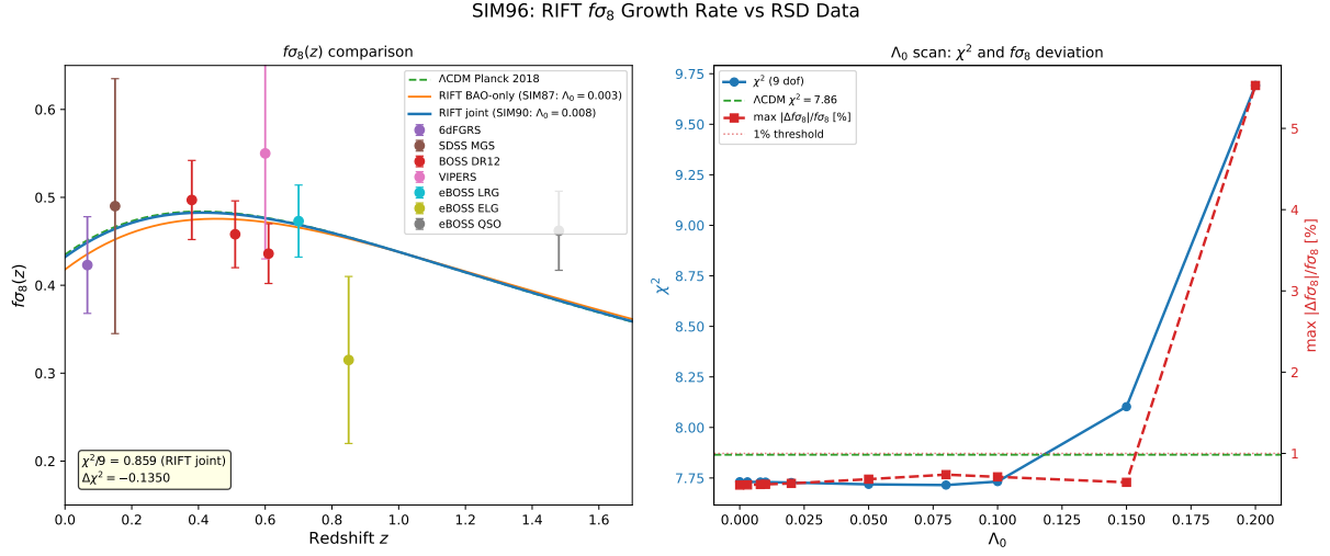
Figure 6: Left : f\sigma_8(z) predictions for RIFT joint best-fit, RIFT BAO-only, and \Lambda CDM Planck 2018, compared to the gold-sample RSD compilation (Sim 96). RIFT at joint best-fit gives \chi^2/\text{dof} = 0.86 , \Delta\chi^2(\text{RIFT} - \Lambda\text{CDM}) = -0.14 . Right : \Lambda_0 scan showing \chi^2 (blue) and maximum fractional f\sigma_8 deviation from \Lambda CDM (red). The deviation exceeds 1% only at \Lambda_0 > 0.2 , beyond the Bayesian upper limit from Sim 93 ( \Lambda_0 < 0.095 at 95% CL).
