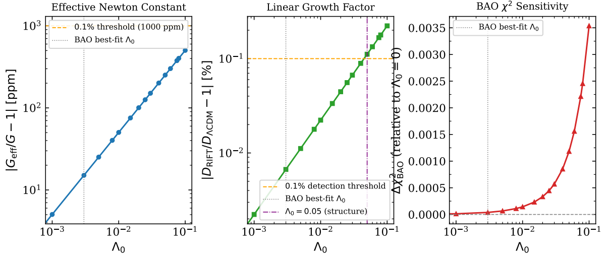
RIFT Coupling-Strength Sensitivity Scan (Sim 91) [ H_0 = 67.6 , \Omega_m = 0.312 ]
