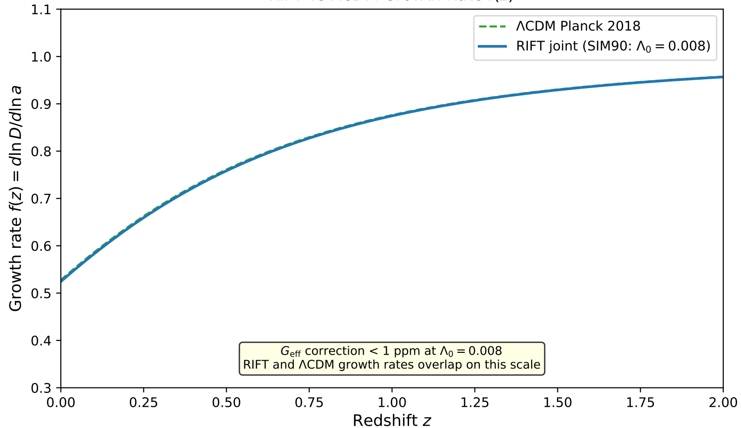
RIFT vs \Lambda CDM Growth Rate f(z)
