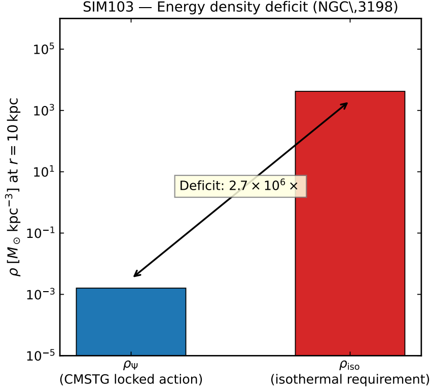
Figure 5: Energy density deficit at galactic scale (SIM103). The locked-action CMSTG scalar density \rho_\Psi (blue bar) vs the isothermal halo requirement \rho_{\text{iso}} (red bar) at r = 10 \text{ kpc} for NGC 3198 ( v_{\text{flat}} = 157 \text{ km s}^{-1} ). The deficit is 2.7 \times 10^6 \times . A direct coupling \beta \approx 4.9 \approx 1,600 \times \Lambda_0 would be required to supply the missing density, far exceeding the cosmological bound \Lambda_0 \lesssim 0.095 .
