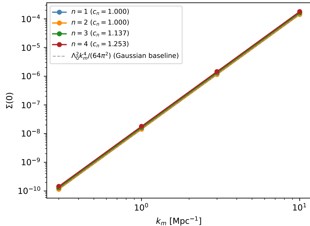
Stretched-exponential family
