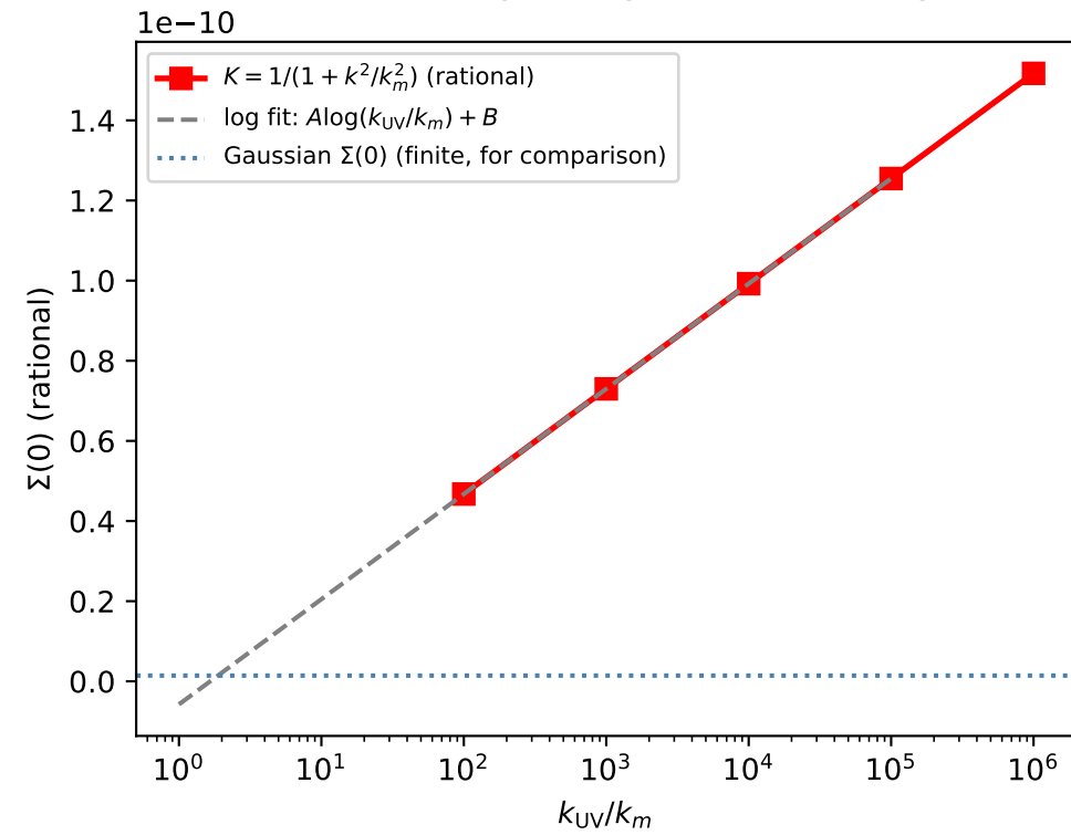
Rational kernel: log-divergent (FAILS to regulate)
