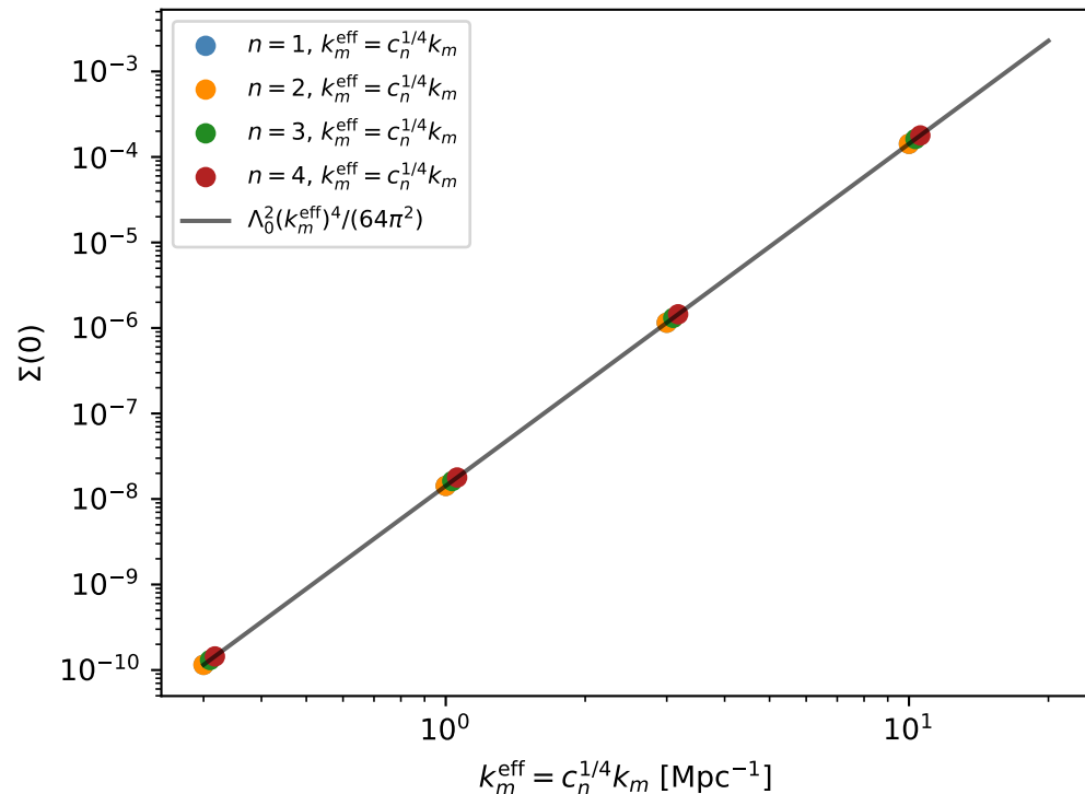
Universal collapse after rescaling
