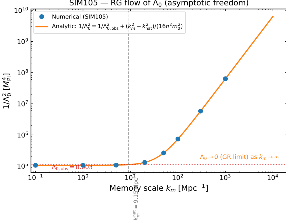
Figure 3: RG flow of 1/\Lambda_0^2 as a function of memory scale k_m (SIM105). Numerical result (blue circles) vs analytic formula (13) (orange solid). The IR fixed value \Lambda_{0\text{obs}} = 0.003 is marked; the naturalness anchor k_m^{\text{nat}} = 9.15 \text{ Mpc}^{-1} and the UV limit \Lambda_0 \rightarrow 0 (horizontal dashed line) are indicated. No Landau pole exists for any k_m \geq 0 .
