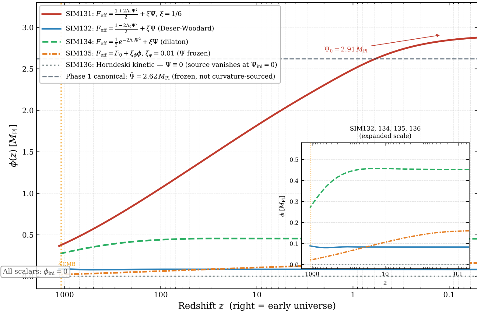
Theorem 1: curvature-sourced scalars initialized at \phi_{\text{ini}} = 0 grow monotonically (violates Eq. (2))
