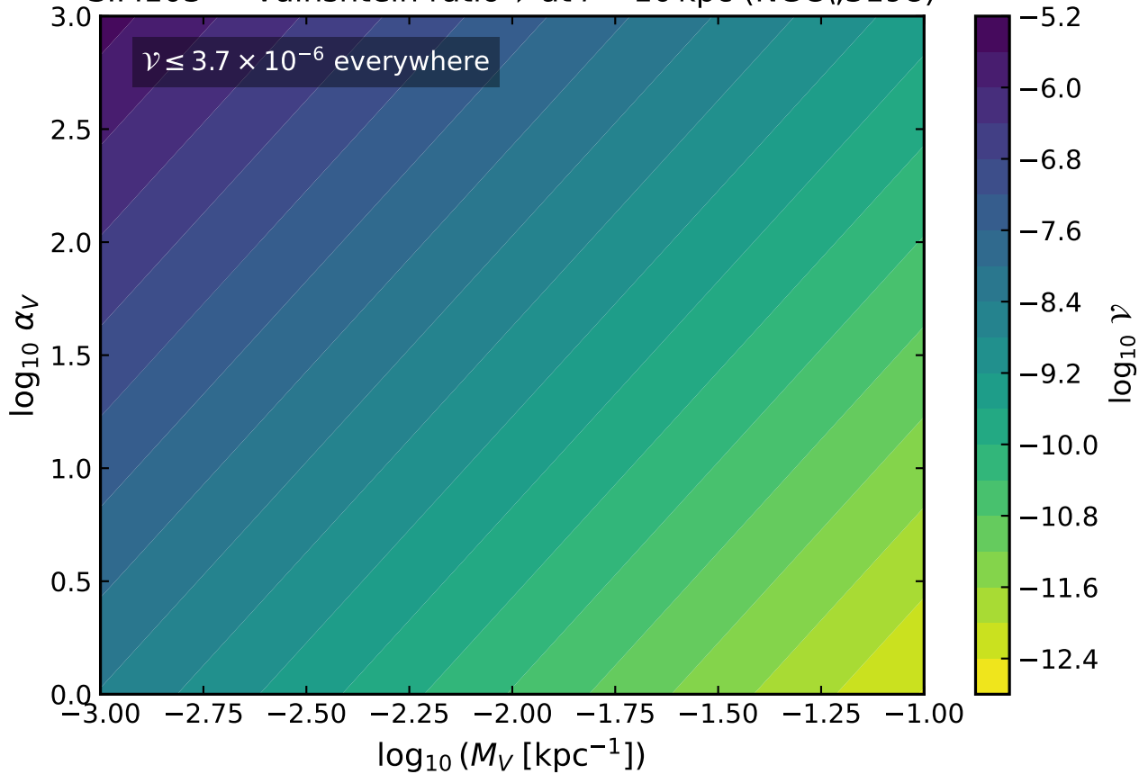
SIM103 — Vainshtein ratio \mathcal{V} at r = 10 kpc (NGC\,3198)
