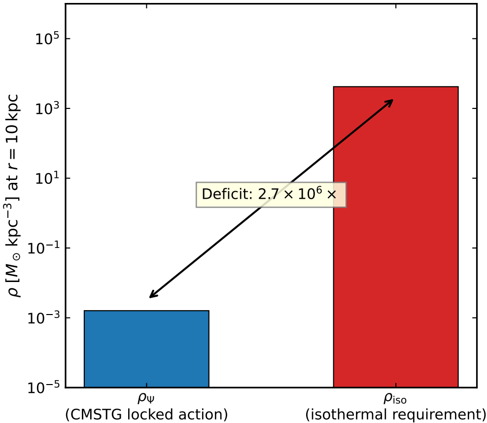
SIM103 — Energy density deficit (NGC\,3198)
