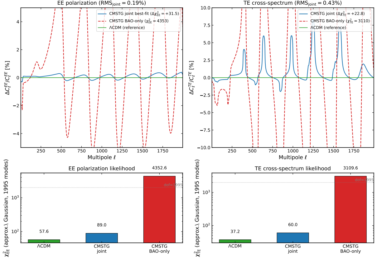
Figure 5: CMSTG vs \Lambda CDM CMB EE and TE power spectra (Sim 95). Top : fractional deviation \Delta C_\ell^{EE}/C_\ell^{EE} and \Delta C_\ell^{TE}/C_\ell^{TE} for the CMSTG joint best-fit relative to Planck 2018. RMS deviations are 0.19% (EE) and 0.43% (TE). Bottom : approximate polarization \chi^2 for the three cosmologies. The BAO-only CMSTG best-fit (A) shows large tension ( \chi_{EE}^2 = 4353 ), while the joint best-fit (B) is statistically consistent with \Lambda CDM (C).
