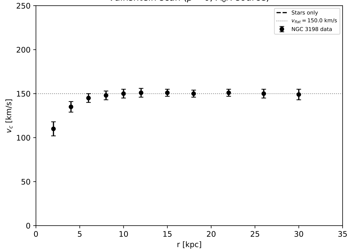
Vainshtein scan ( \beta = 0 , \Lambda_0 R source)
