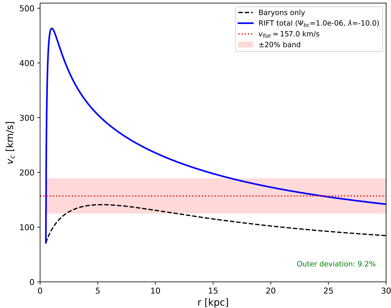
NGC3198 — Best-fit rotation curve (best within cosmo+energy bounds)
