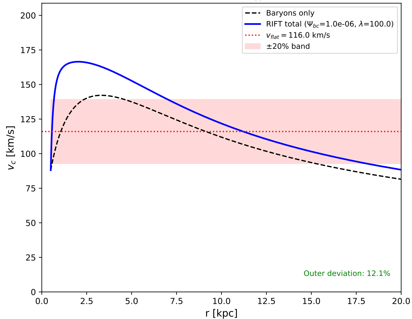
NGC6503 — Best-fit rotation curve (best within cosmo+energy bounds)
