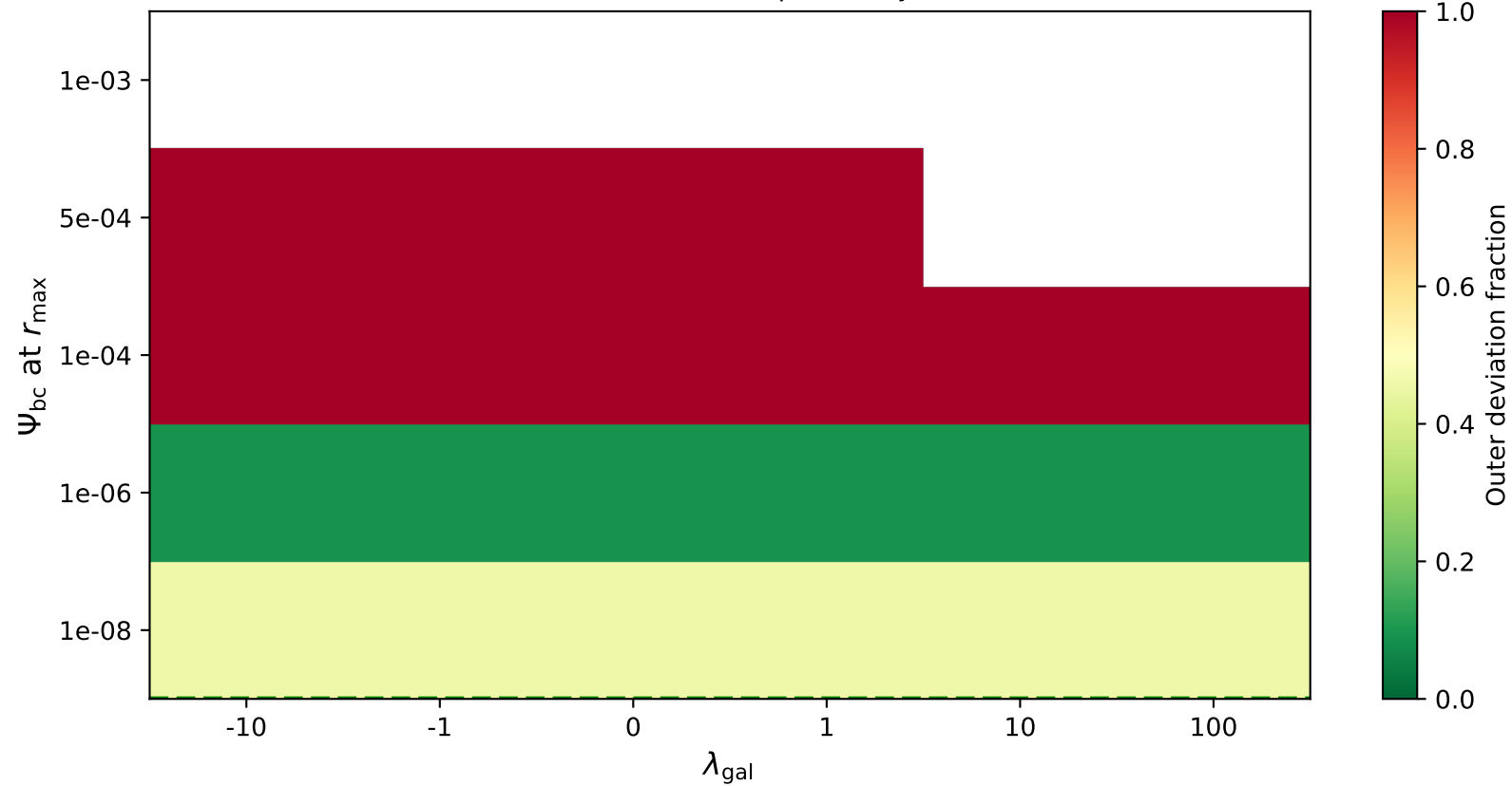
NGC3198 — Outer |v_c - v_{flat}|/v_{flat} (within cosmo+energy bounds) Green = flat (20% tol), Red = discrepant, Gray = bound violated
