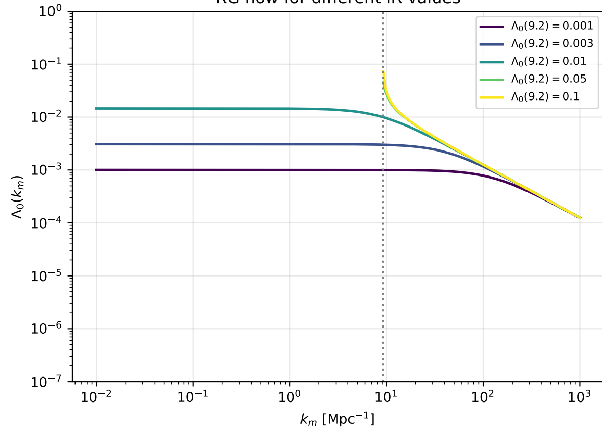
RG flow for different IR values
