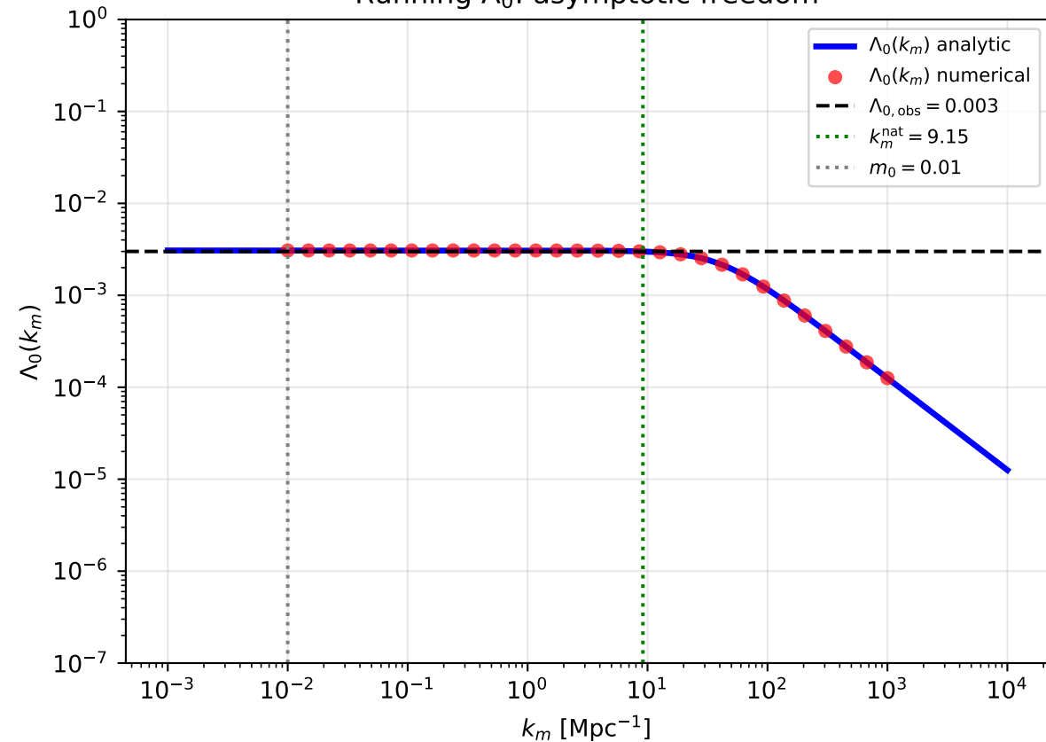
Running \Lambda_0 : asymptotic freedom
