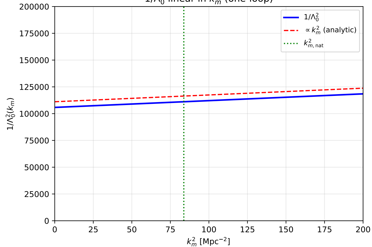
1/\Lambda_0^2 linear in k_m^2 (one-loop)
