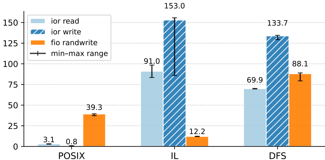
Median bandwidth (GiB/s)
