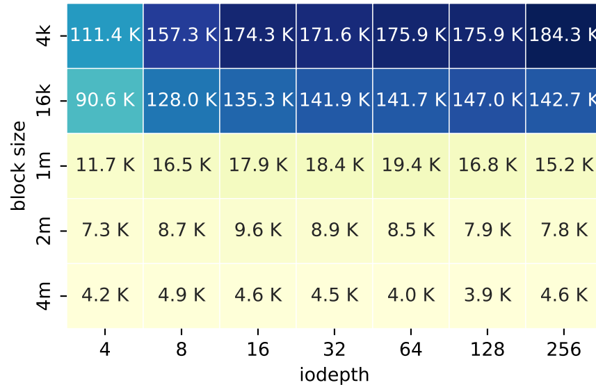
fio single-job random write
