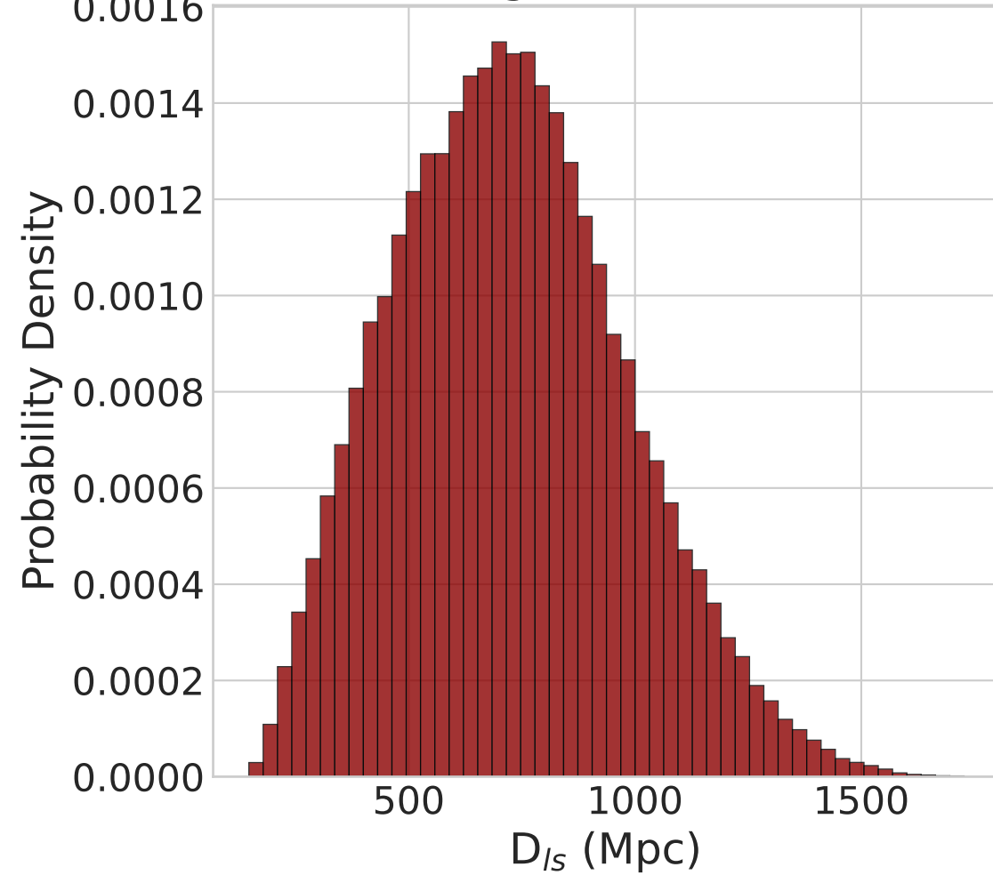
Lens-Source Angular Diameter Distance
