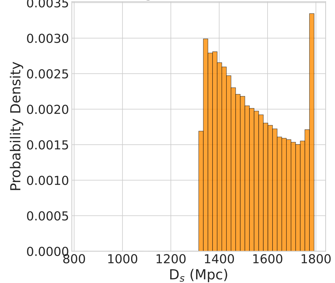
Source Angular Diameter Distance
