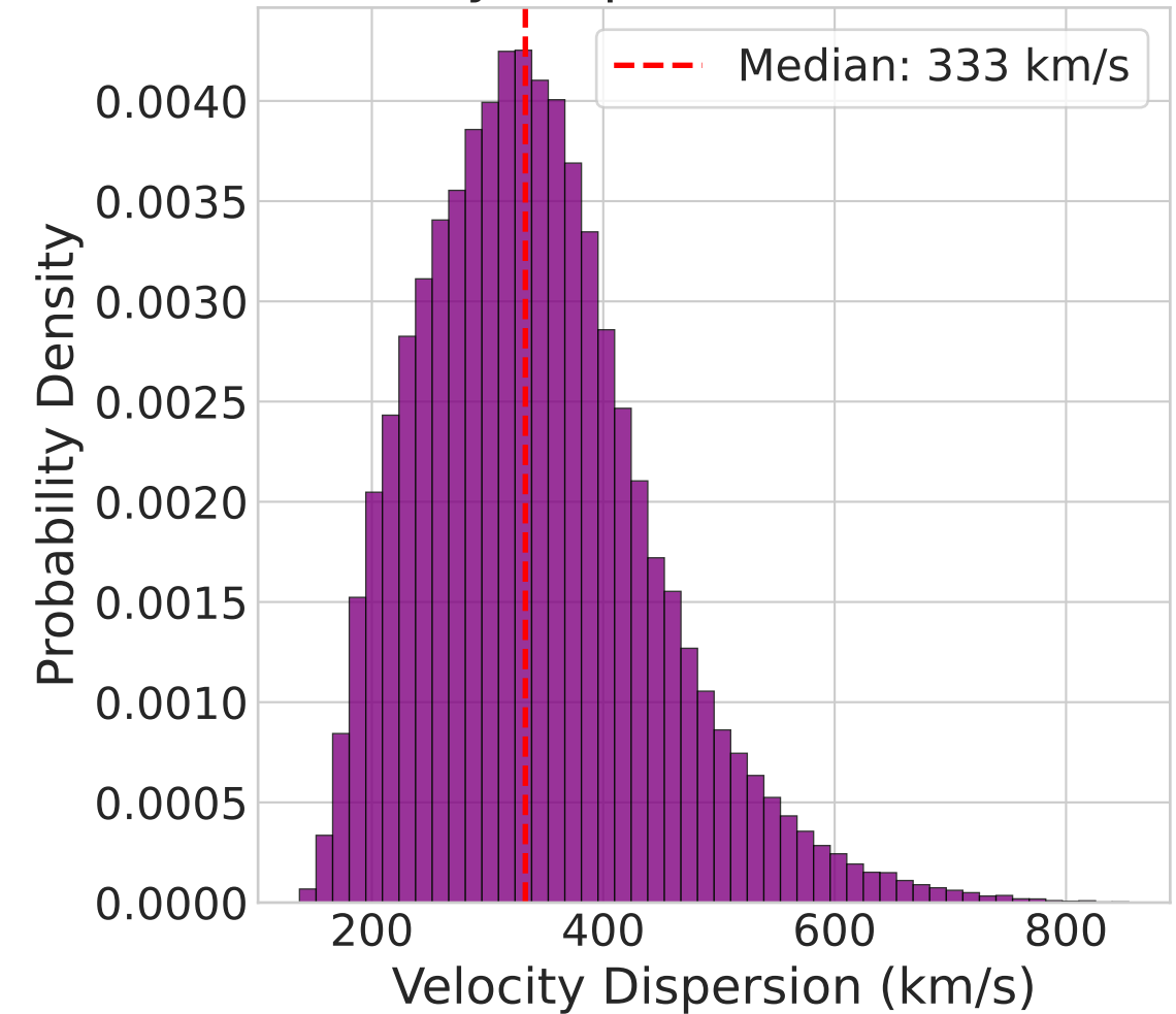
Velocity Dispersion Distribution
