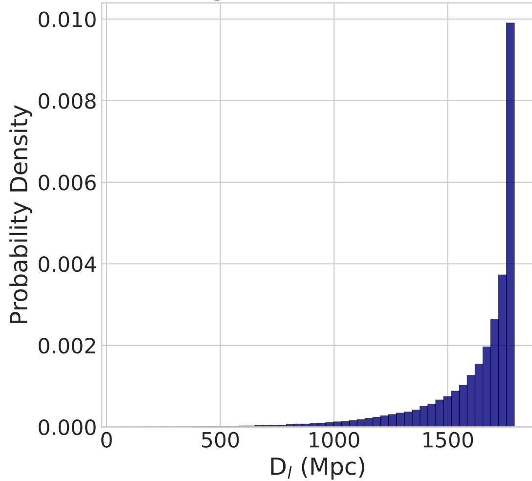
Lens Angular Diameter Distance
