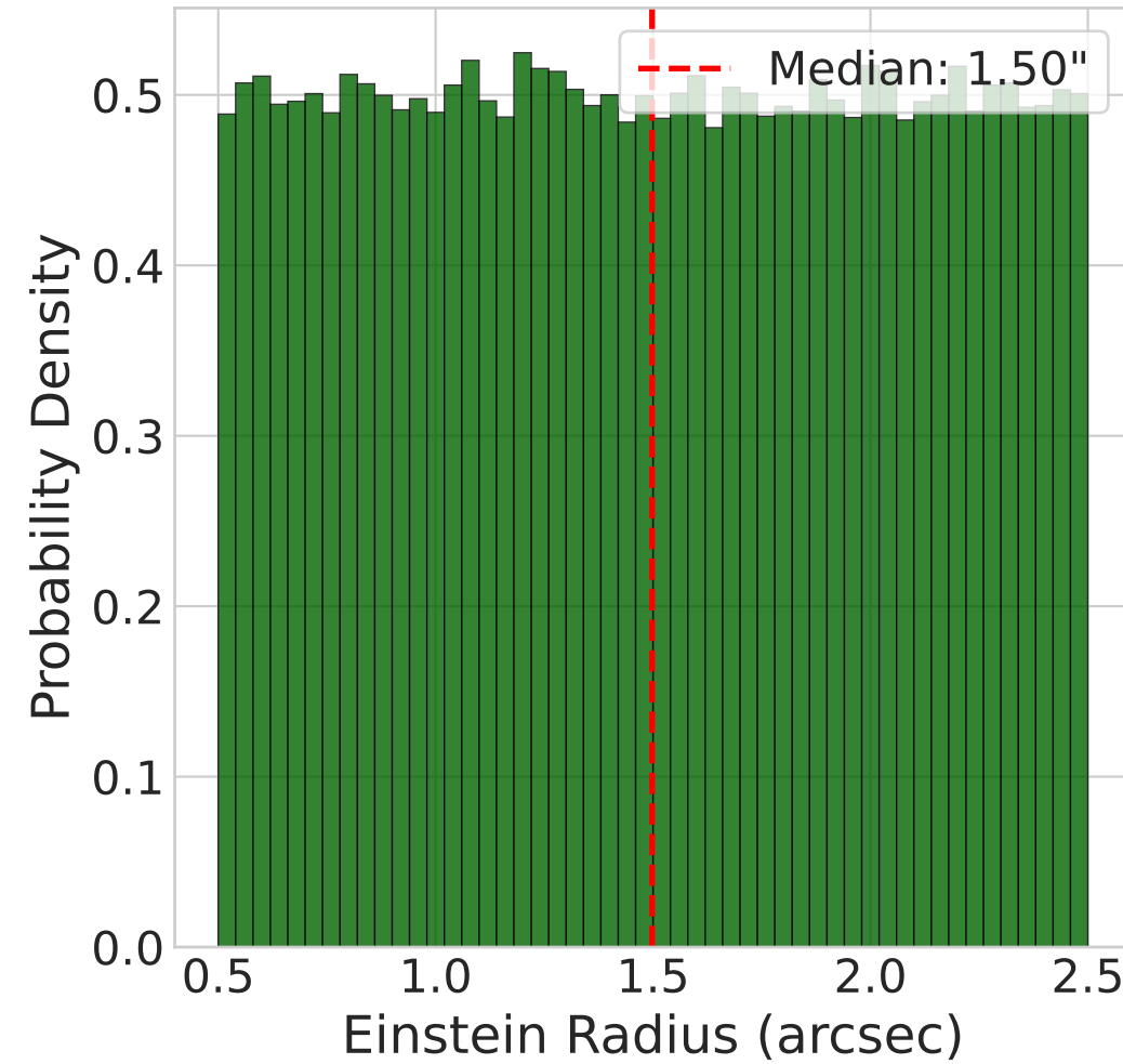
Einstein Radius Distribution
