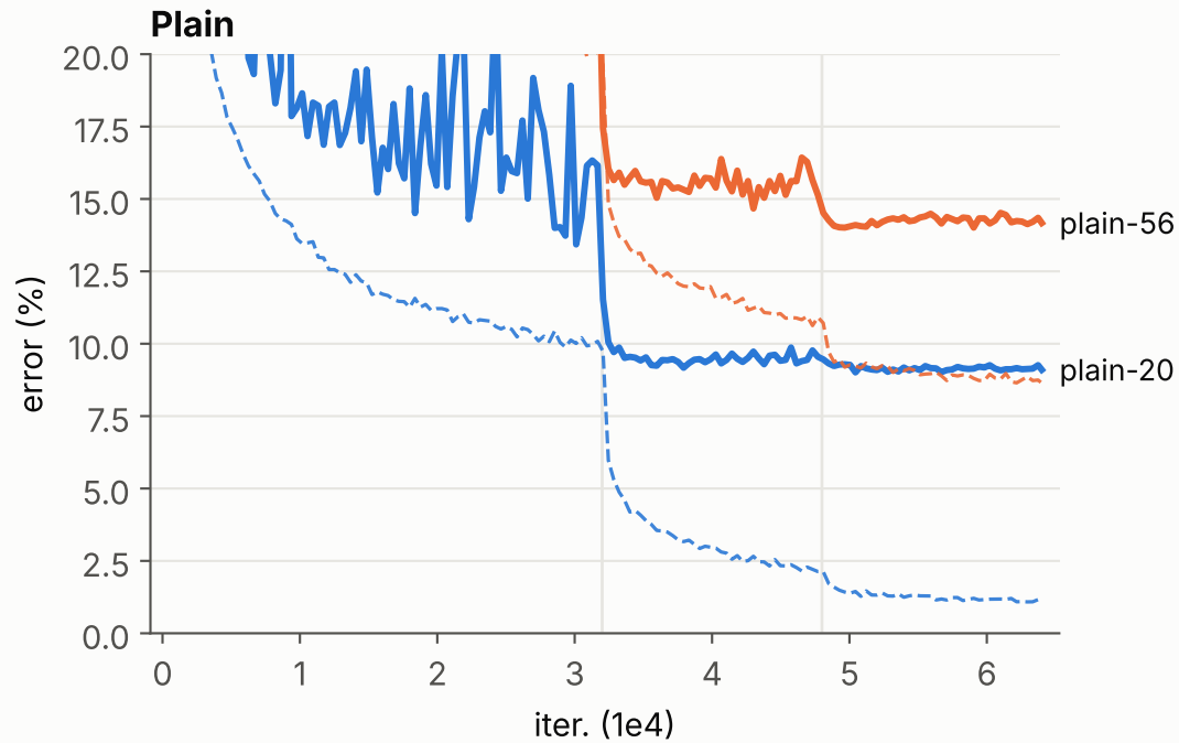
CIFAR-10 — our runs (dashed: training error, bold: test error)
